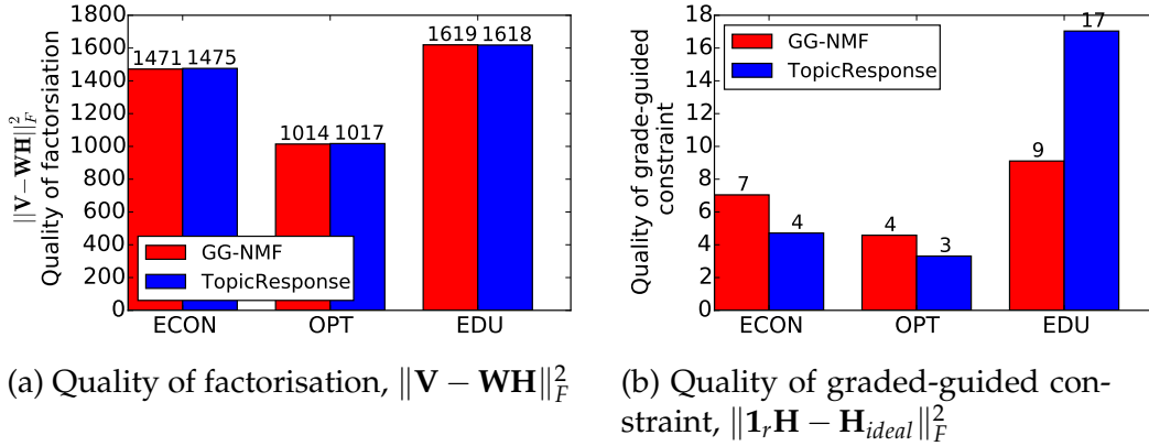
Figure 5.3: Performance of GG-NMF and TopicResponse in terms of \|\mathbf{V} - \mathbf{WH}\|_F^2 and \|\mathbf{1}_r \mathbf{H} - \mathbf{H}_{ideal}\|_F^2 ; Smaller is better.
