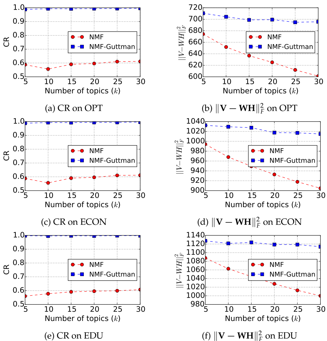
Figure 4.8: Comparison of NMF and NMF-Guttman in terms of CR and \|V - WH\|_F^2 with varying the number of topics ( k ).
