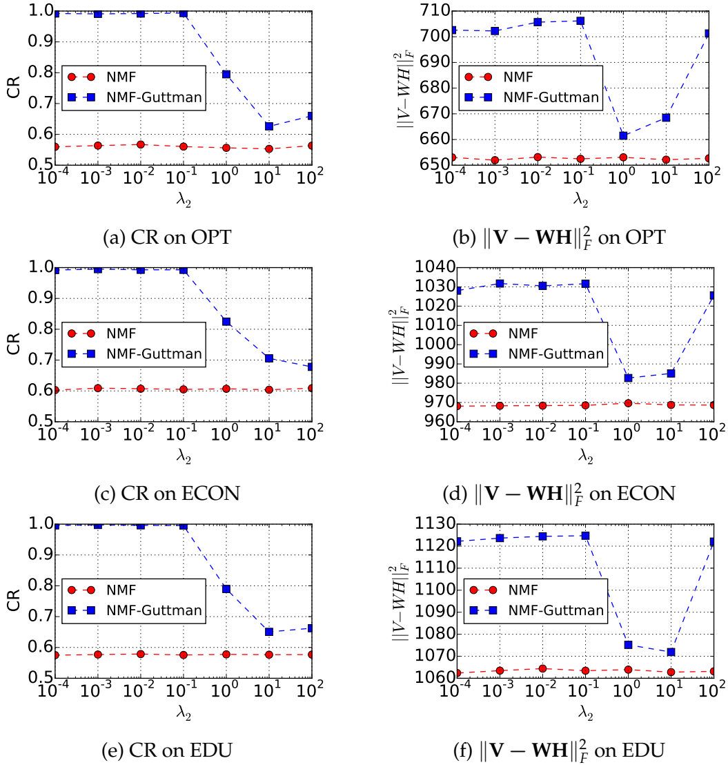
Figure 4.7: Comparison of NMF and NMF-Guttman in terms of CR and \|V - WH\|_F^2 with varying \lambda_2 .
