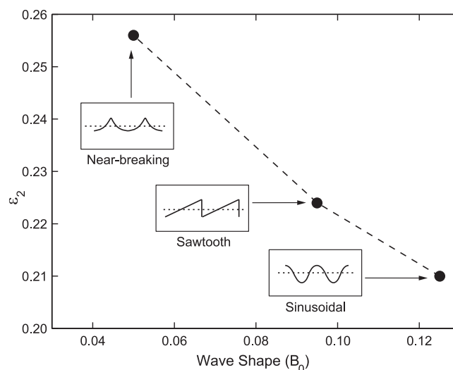
Figure 15. Hypothesized wave shape effect on Snyder's \epsilon_2 coefficient.
