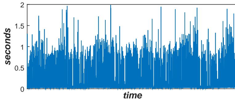
Figure 5.16: Response time for on-demand auto-scaling on Amazon
