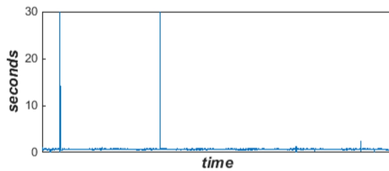
Figure 5.14: Response time of one spot type auto-scaling with various percentage of on-demand resources and on-demand bidding strategy
