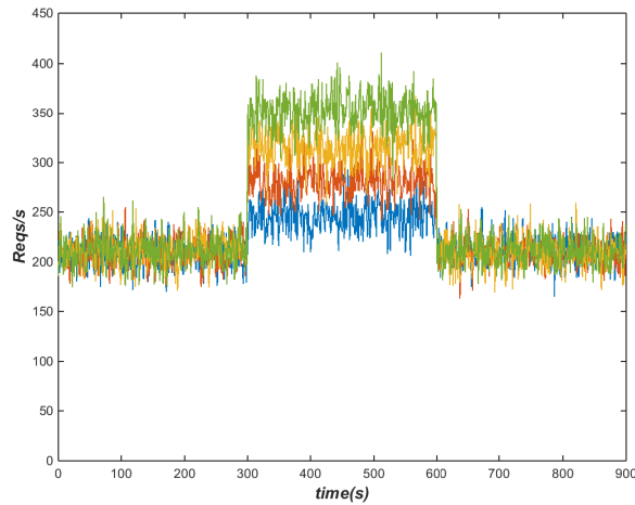
Figure 6.7: The workloads with flash crowds range from 117% to 183% of the normal load experiments. We first generated the background workloads for the Ireland and Tokyo data centers respectively with average incoming rates of 105 requests/s and 210 requests/s. To test the performance of the approach during resource failures in North Virginia data center, we generated a workload with average request rate of 210 requests/s. For flash crowds cases, we created four workloads with different levels of flash crowds as shown in Figure 6.7. Each workload experiences a total five minutes of flash crowd. The peaks of the flash crowds range from 117% to 183% of the normal load. All the workloads last for 15 minutes and suffer either server failures or flash crowds starting from the 300s time point for 300 seconds. We particularly chose the length of 300 seconds because it is the default value of the waiting time for server booting in Amazon Auto-scaling Service. In this way, we can emulate the situations that a commercial auto-scaler solely manages the application and demonstrate its resulted application performances during the overloading periods.
