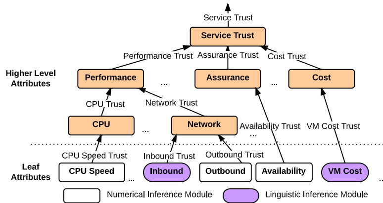
Figure 3.4: Example of Hierarchical Fuzzy Inference System for Trust Evaluation
