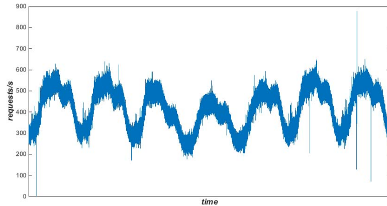
Figure 5.9: The English Wikipedia workload from Sep 19th 2009 to Sep 26th 2009
