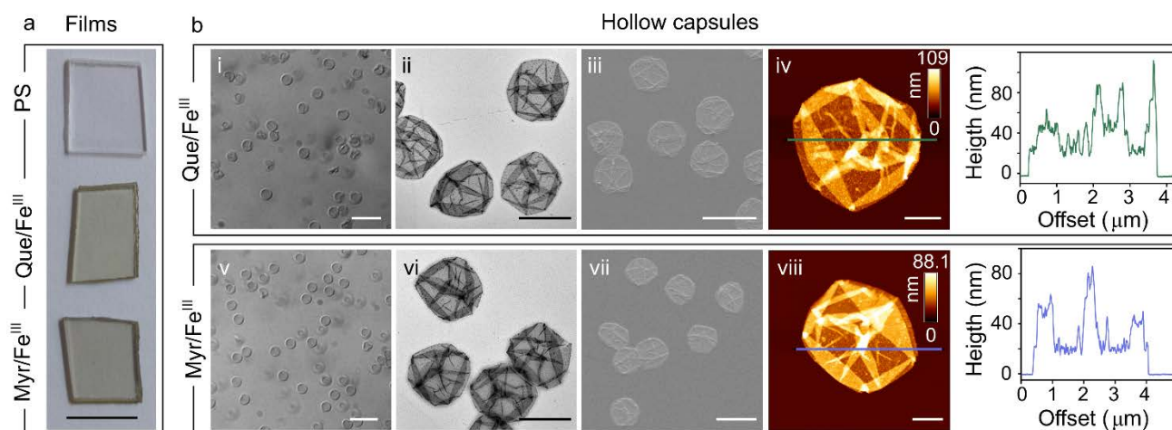
Fig. 1 a) Characterization of flavonoid/Fe III films on planar PS substrates (scale bar 1 cm). From top to bottom: a piece of uncoated PS, PS coated with a Que/Fe III film, and PS coated with a Myr/Fe III film (five deposition cycles, respectively). b) Characterization of Que/Fe III and Myr/Fe III hollow capsules that were obtained after film formation on PS particles and subsequent PS removal. From left to right: differential interference contrast (DIC) microscopy (i, v), transmission electron microscopy (TEM) (ii, vi), scanning electron microscopy (SEM) (iii, vii) and atomic force microscopy (AFM) (with the height profile corresponding to the cross section indicated in green (iv) and blue (viii)) images. Scale bars are 10 \mu m (i, v), 3 \mu m (ii, vi), 5 \mu m (iii, vii), and 1 \mu m (iv, viii).
