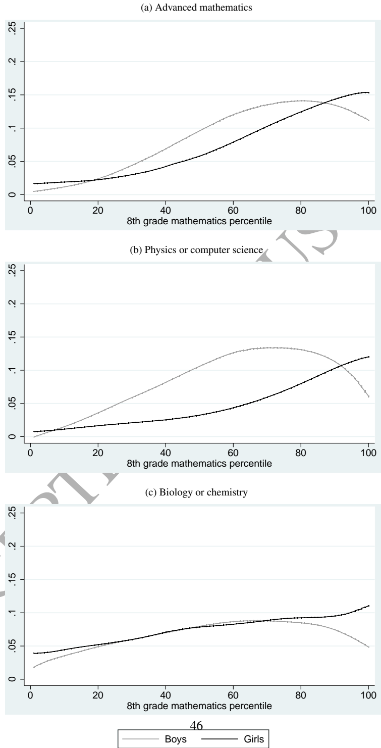
Figure A3: Differences in share of students selecting advanced science or mathematics electives between highest and lowest family income by gender and eighth-grade mathematical achievement
