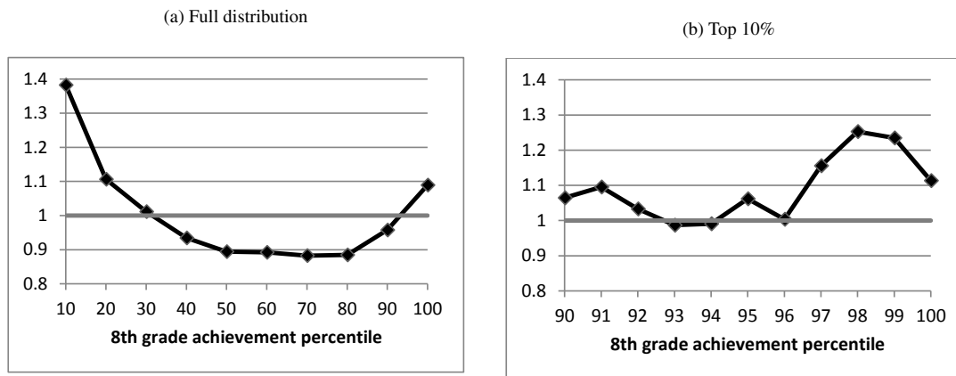
Figure 2: Male/female ratio by eighth-grade mathematics achievement rank
