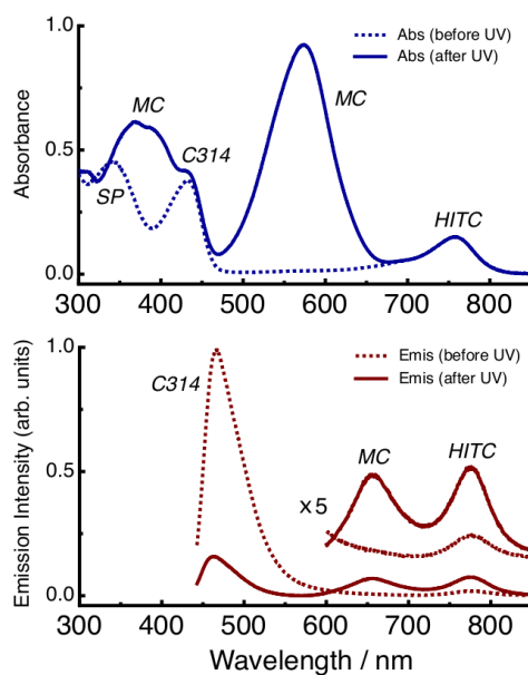
Fig. 3 Absorption (top panel) and emission (bottom panel, \lambda_{ex} = 435 nm) spectra of the C314+SP/MC+HITC PMMA sample, before and after UV irradiation.
