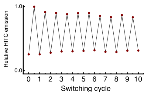
Fig. 4 Relative intensity of the HITC emission following C314 excitation in the C314+SP/MC+HITC PMMA sample when switching between SP and MC dominant populations using UV and visible light irradiation cycles.
