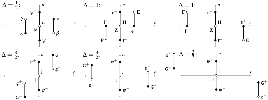
FIGURE 2. The weights (n, e) of the fields generating the extended chiral algebras along with the weights of \mathfrak{gl}(1|1) itself (we label the weights by the corresponding fields). White weights are bosonic and black weights are fermionic. The first weight diagram corresponds to the direct sum of a \beta\gamma ghost system with a complex fermion, the second to \widehat{\mathfrak{sl}}(2|1)_1 , the third to \widehat{\mathfrak{sl}}(2|1)_{-1/2} and the last three to the W -algebras of Section 5.4.
