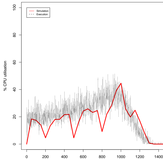
Figure 3.10: Predicted and actual CPU utilisation of the AS server with 300 simultaneous sessions in Experiment 1.
