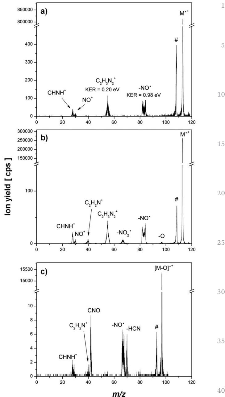
Fig. 6 VG ZAB2-SEQ tandem mass spectra of cations of 4(5)-nitroimidazole formed via electron ionization (Fig. 3c): (a) MIKE scan of M^{++} , and high-energy CID at 6 keV with helium of (b) M^{++} and (c) [M - O]^+ . # is an artefact.
