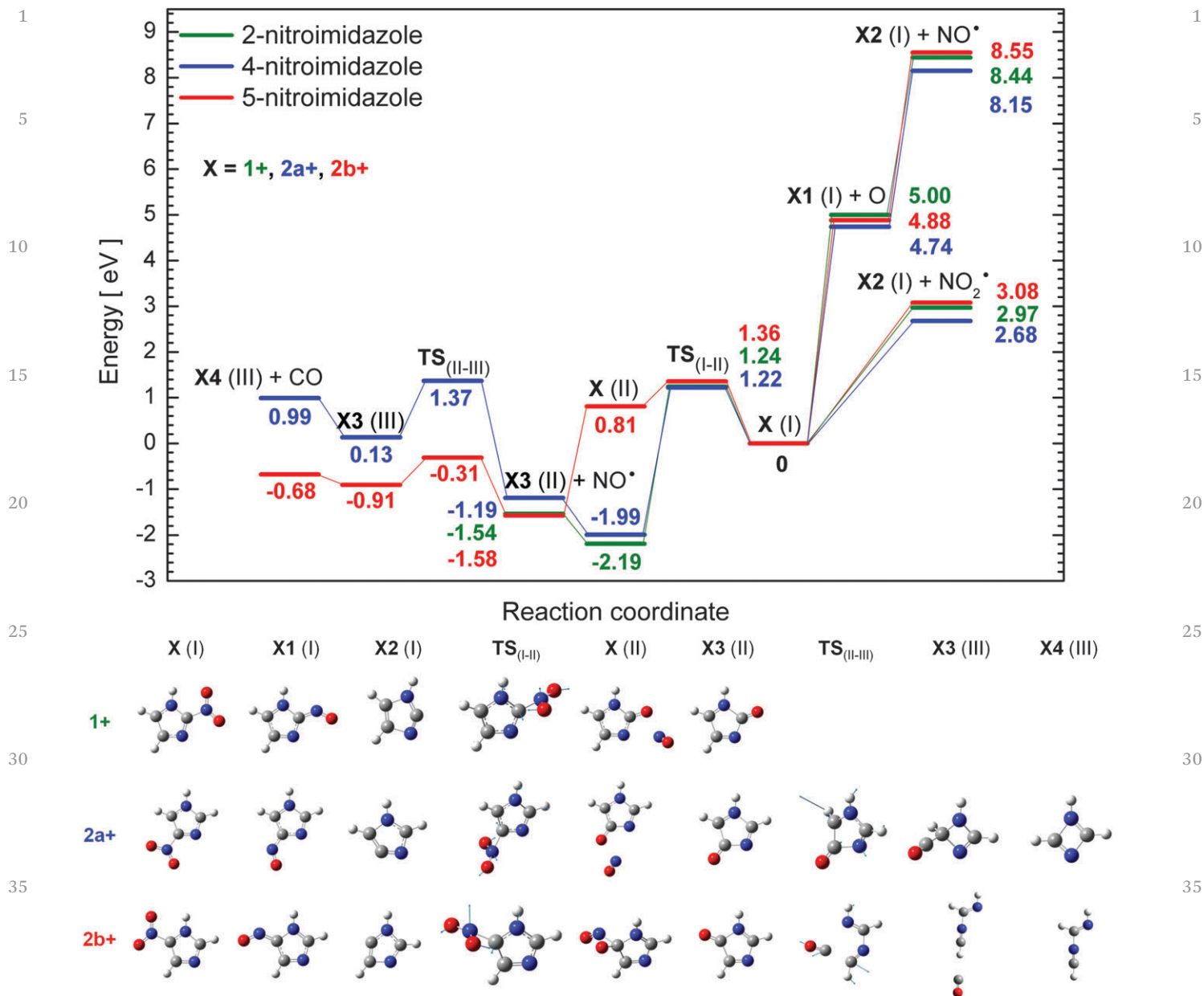
Fig. 7 M062x/6-311+G(d,p) calculated potential energy diagram for decomposition of the M^{\bullet+} radical cation, where M = 2-nitroimidazole (green), 4-nitroimidazole (blue), and 5-nitroimidazole (red). Calculated energy values in eV include a zero-point energy correction. The blue arrows in the respective TS show the displacement vectors.
