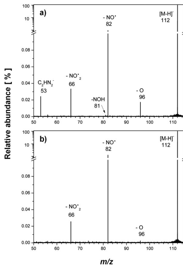
Fig. 10 LTQ-FT EID of ESI generated [M-H]^- of: (a) 2-nitroimidazole at 21 eV electron energy and (b) 4(5)-nitroimidazole at 31 eV electron energy.
