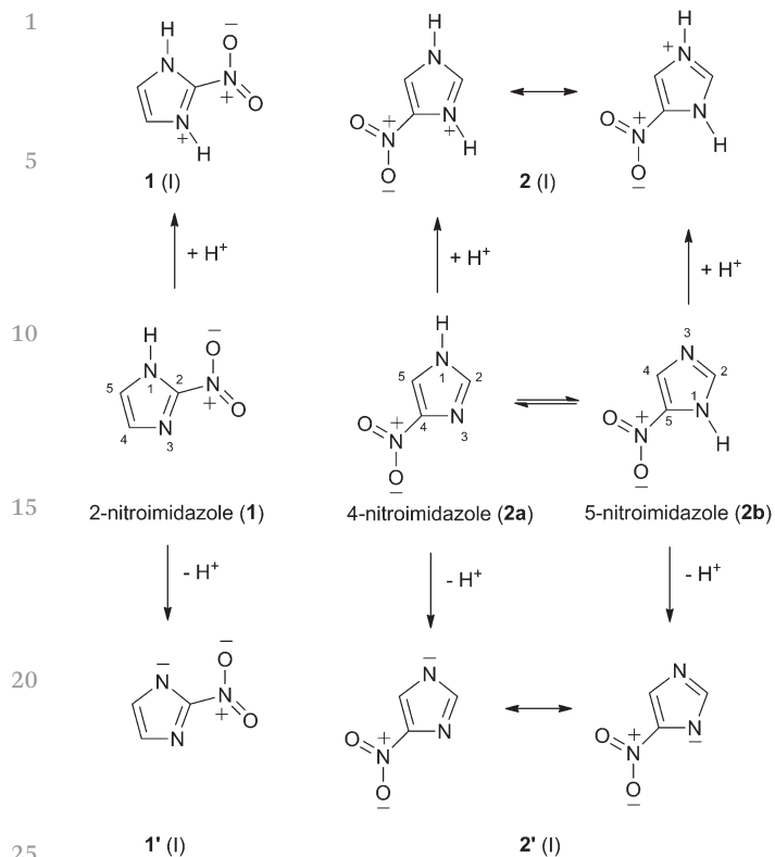
Fig. 1 Structures of nitroimidazole compounds investigated: 2-nitroimidazole ( 1 ), 4-nitroimidazole ( 2a ), 5-nitroimidazole ( 2b ). 2a and 2b are annular tautomers which produce the same [M + H]^+ and [M - H]^- upon N-protonation or N-deprotonation respectively.
