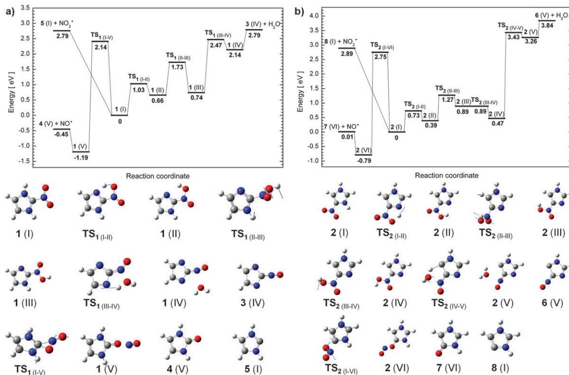
20 Fig. 4 M062x/6-311+G(d,p) calculated potential energy diagram for decomposition of the [M + H] + ion, where M = (a) 2-nitroimidazole and (b) 4(5)-nitroimidazole. Calculated energy values in eV include a zero-point energy correction. The blue arrows in the respective TS show the displacement vectors.
