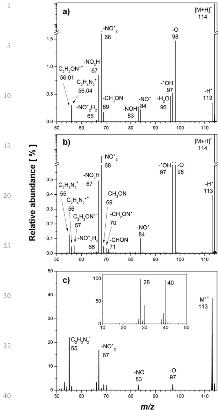
Fig. 5 LTQ-FT EID spectra of ESI generated [M + H]^+ of (a) 2-nitroimidazole and (b) 4(5)-nitroimidazole at electron energy of 21 eV; and (c) VG ZAB2-SEQ electron ionization mass spectrum of 4(5)-nitroimidazole with an electron energy of \sim 70 eV.
