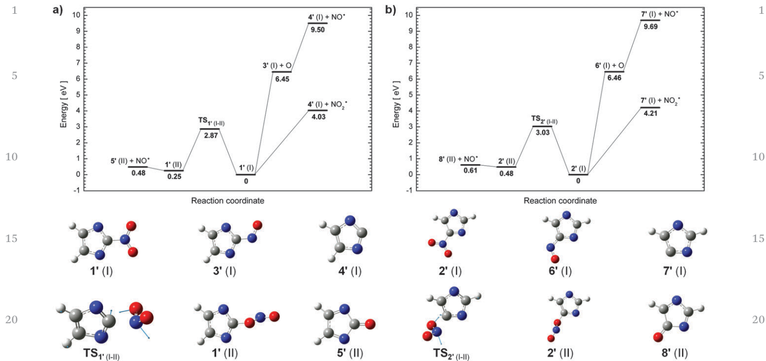
Fig. 9 M062x/6-311+G(d,p) calculated potential energy diagram for decomposition of the [M-H]^- anion, where M = (a) 2-nitroimidazole and (b) 4(5)-nitroimidazole. Calculated energy values in eV include a zero-point energy correction. The blue arrows in the respective TS show the displacement vectors.
