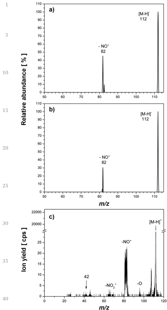
Fig. 8 LTQ-FT Low-energy CID of [M-H]^- of: (a) 2-nitroimidazole and (b) 4(5)-nitroimidazole. Panel (c) shows VG ZAB2-SEQ high-energy CID of [M-H]^- of 4(5)-nitroimidazole in air.
