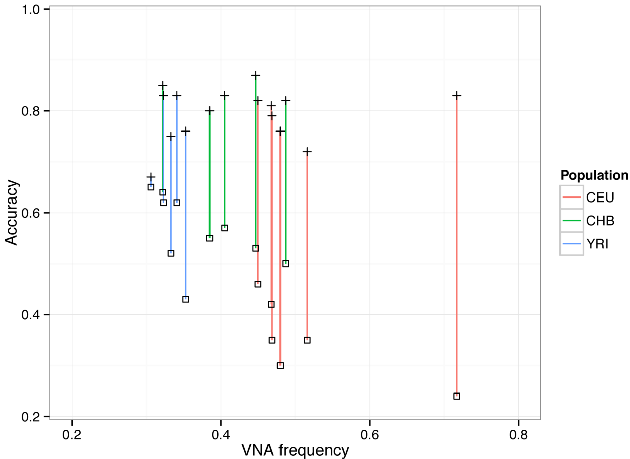
Fig 3. Analysis of ref+ pipeline accuracy. Each vertical line represents one individual, with the plus (+) point representing the ref+ pipeline and the square point representing the GRC pipeline.
