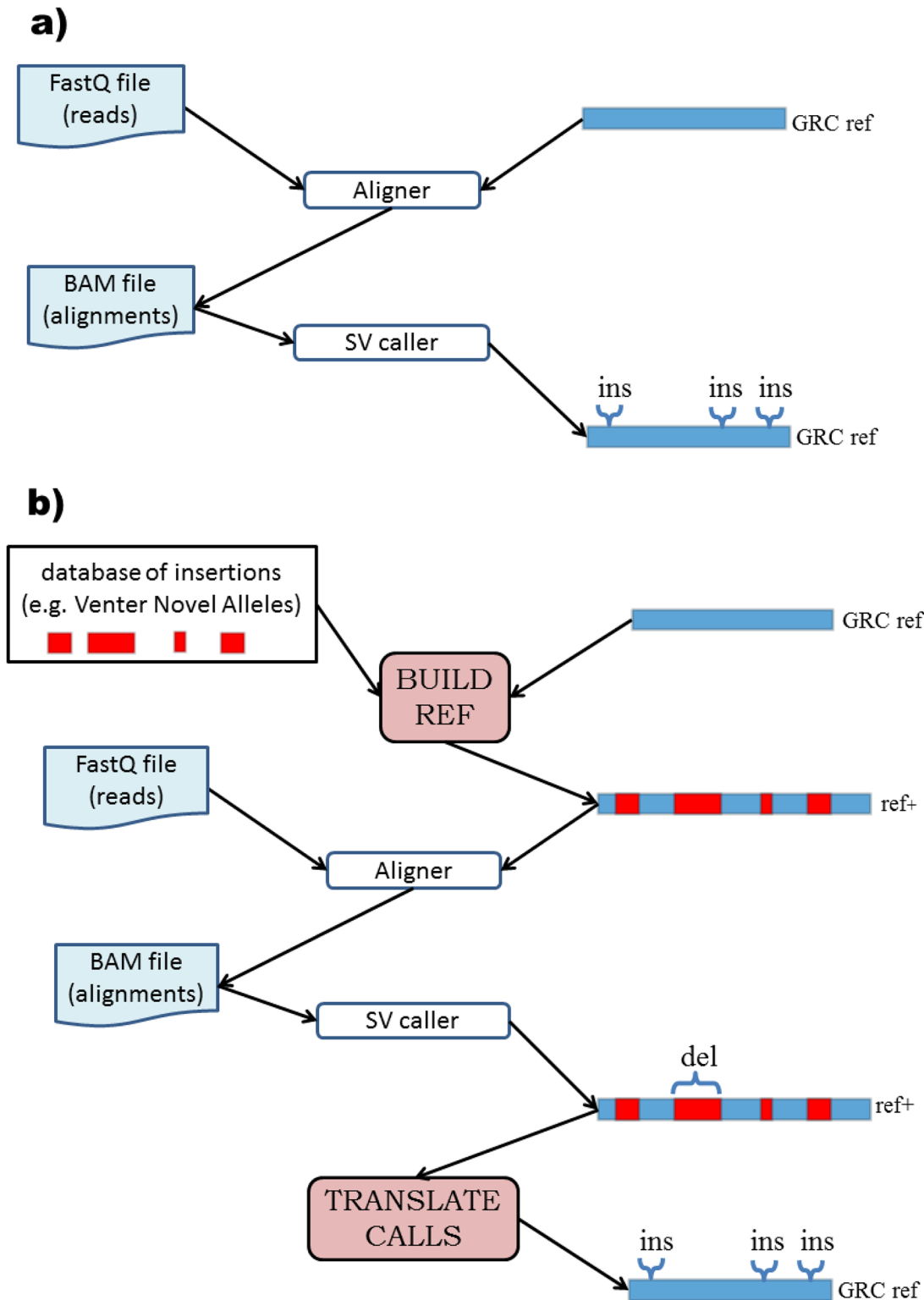
Fig 1. Method workflow. a) In a traditional SV calling pipeline the reads are first aligned against the GRC reference and the alignments are passed to an SV caller, which annotates regions of the GRC reference as being inserted/deleted. b) Our approach is composed of two additional components. BUILD_REF takes a set of sequences to be inserted and modifies the GRC reference genome (e.g. hg18) by inserting the sequences into their prescribed locations, obtaining a new genome (ref+). We next align the reads to ref+ and run a SV caller. The TRANSLATE_CALLS component then modifies the resulting calls so that they become calls relative to the GRC reference, not ref+.
