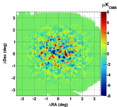
Fig. 4: Preliminary first season E-mode polarization map for one of three observation patches, with approximately 1700 hours of observation time. (Color figure online)
