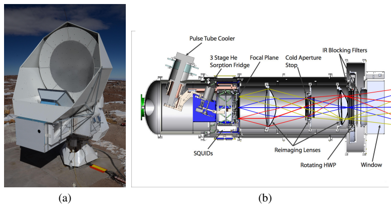
Fig. 1: (a) The Huan Tran Telescope (b) A cross-sectional drawing of the POLARBEAR cryogenic receiver with major components identified. (Color figure online)
