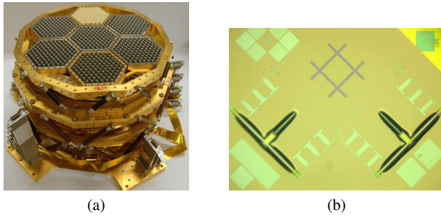
Fig. 2: (a) POLARBEAR’s complete focal plane including lenslets, support structures and wiring. One array module has white alumina instead of silicon lenslets (b) A single pixel, with two TES detectors and slot antenna (Color figure online)
