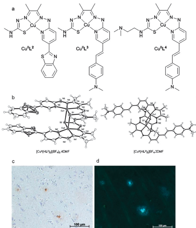
Fig. 11 (a) Structure of complexes [CuL^2] , [CuL^3] , and [CuL^4] . (b) ORTEP (ellipsoids at 40% probability) representations of [Cu^{II}(HL^2)]_2(BF_4)_2 \cdot 4DMF and [Cu^{II}(H_2L^3)](BF_4) \cdot 2DMF with solvent molecules and anions omitted for clarity. The dication dimer, [Cu^{II}(HL^2)]_2(BF_4)_2 \cdot 4DMF contains benzothiazole rings that are disordered over 2 sites (occupancy 0.5). (c) AD human brain sections ( \times 20 magnification) with 1E8 antibody stain and (d) epifluorescence microscopy of CuL^4 binding to A \beta plaques.
