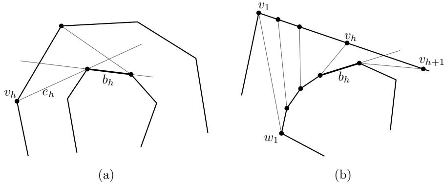
Figure 7.6: (a) If v_h \in b_h^\ominus then B \subseteq e_h^\ominus . (b) If v_{h+1} \in b_h^\ominus then A \cap \bigcup_{i=1}^h b_i^+ = \{v_1, \dots, v_h\} .
