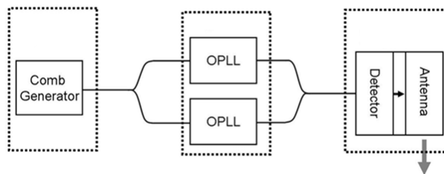
Fig. 1: Millimetre-wave or terahertz generator
