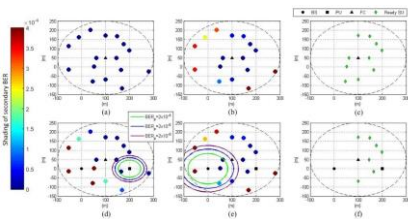
Figure 3. Spectrum sharing for multi-user CR systems for non-overlapping operation, (a) downlink, (b) uplink, and (c) their intersection and for overlapping operation, (d) downlink, (e) uplink, and (f) their intersection
