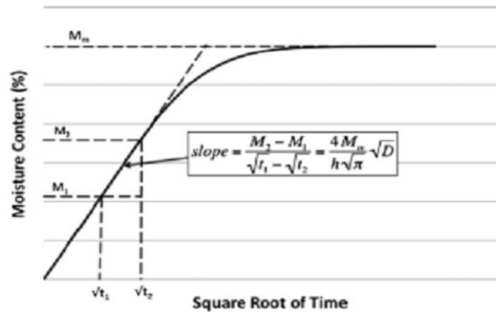
Figure 3: Determination of Diffusion Coefficient (Londhe et al. , 2016)
