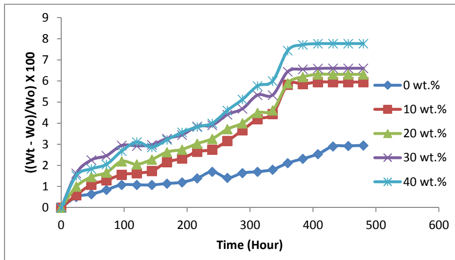
Figure 5: Water Absorption Behavior of Cured neat and Momodical Reinforced Polyester Polymer Composite
