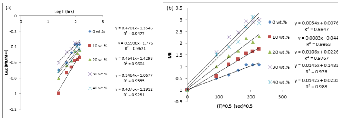
Figure 6: Graphical estimation of diffusivity (a) and mechanism of water absorption (b)
