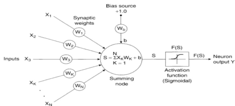
Figure 2: Structure of Artificial Neural Networks
