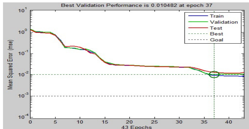
Figure 7 Performance of ANN with 2-5-1-1 topology
