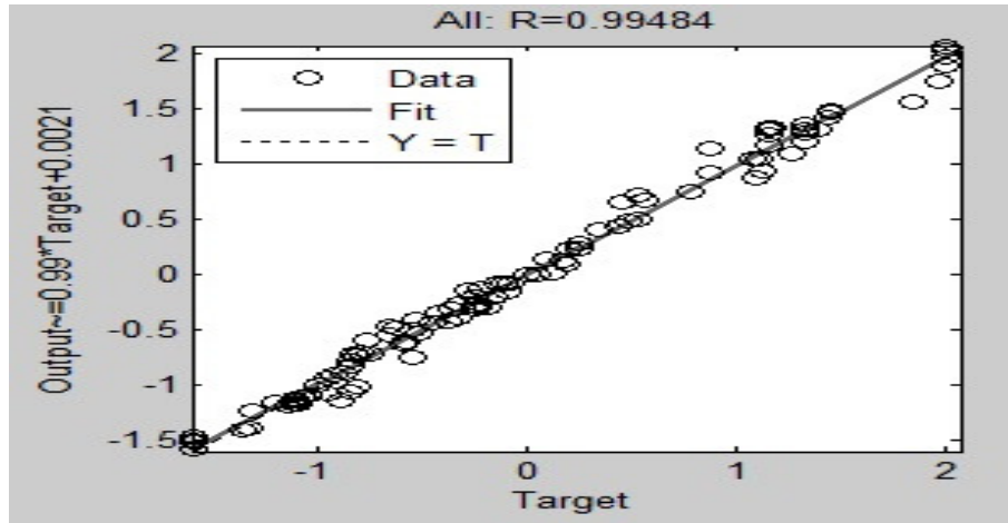
Figure 8 Model Efficiency for 2-5-1-1 Topology
