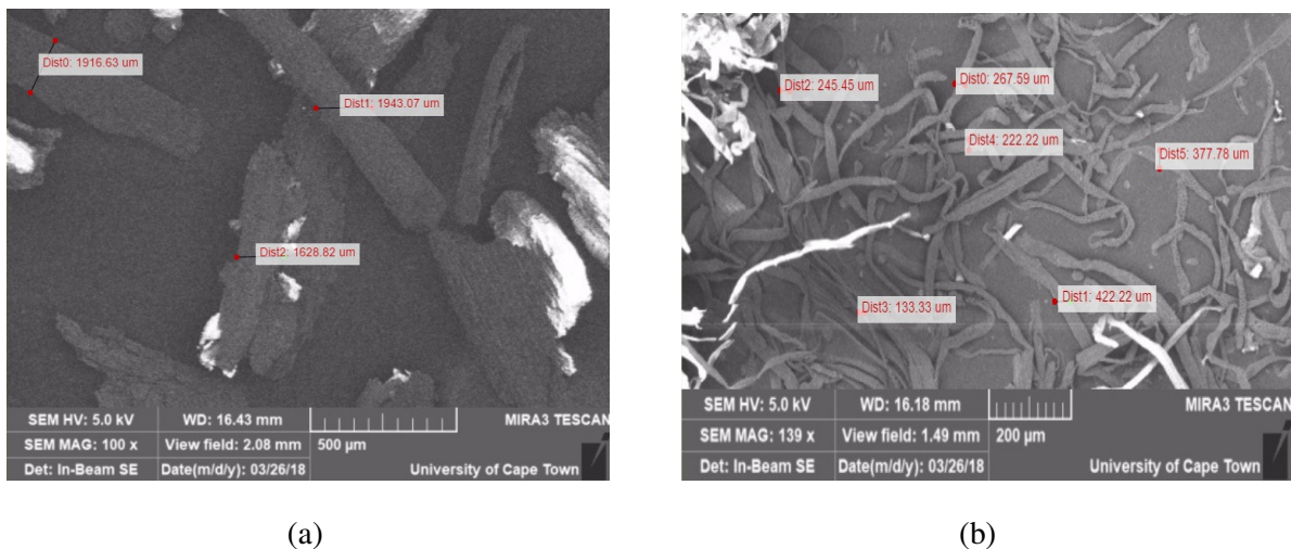
Figure 4: SEM Micrograph of (a) Raw/Untreated and (b) Alkali Treated Momodical Fiber
