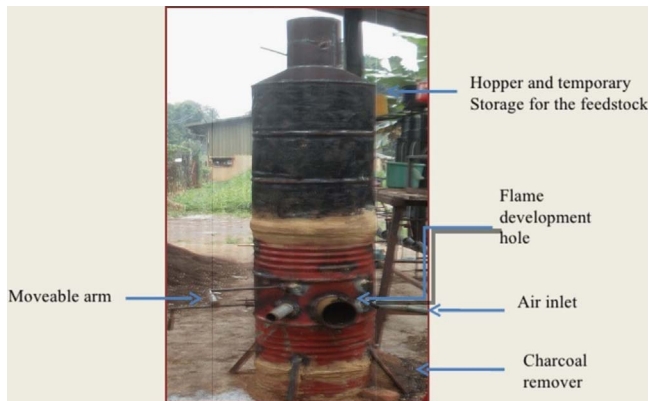
Fig. 2. Fabricated pyrolyzer.
