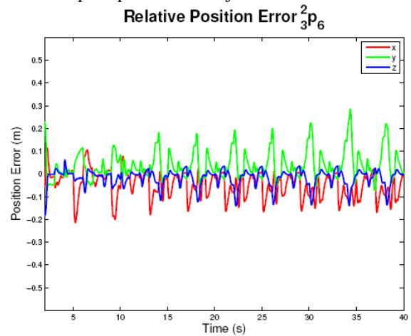
Figure 4. The relative position error {}^2_3 p_6
