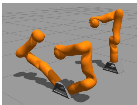
Figure 1. A 3-arm parallel manipulator. Simulation video is shown here: https://youtu.be/w87Ei7Z2Uis .
