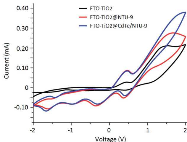
Fig. 7 Cyclic voltammograms for the three types of electrodes in an \text{I}^{3-}/\text{I}^- electrolyte solution: (1) unmodified, (2) NTU-9 modified, and (3) CdTe/NTU-9 modified.
