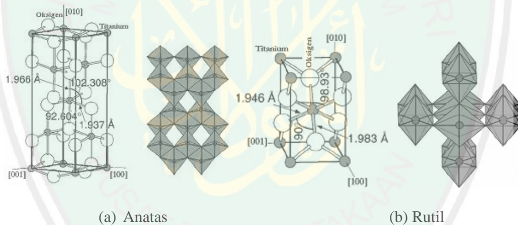
Gambar 2.4 Struktur kristal \text{TiO}_2 : (a) anatase, dan (b) rutil (Diebold, 2003)
