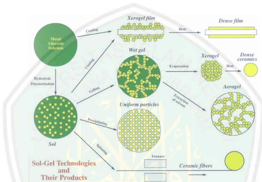
Gambar 2.15 Proses sol-gel (Widodo, 2010)
