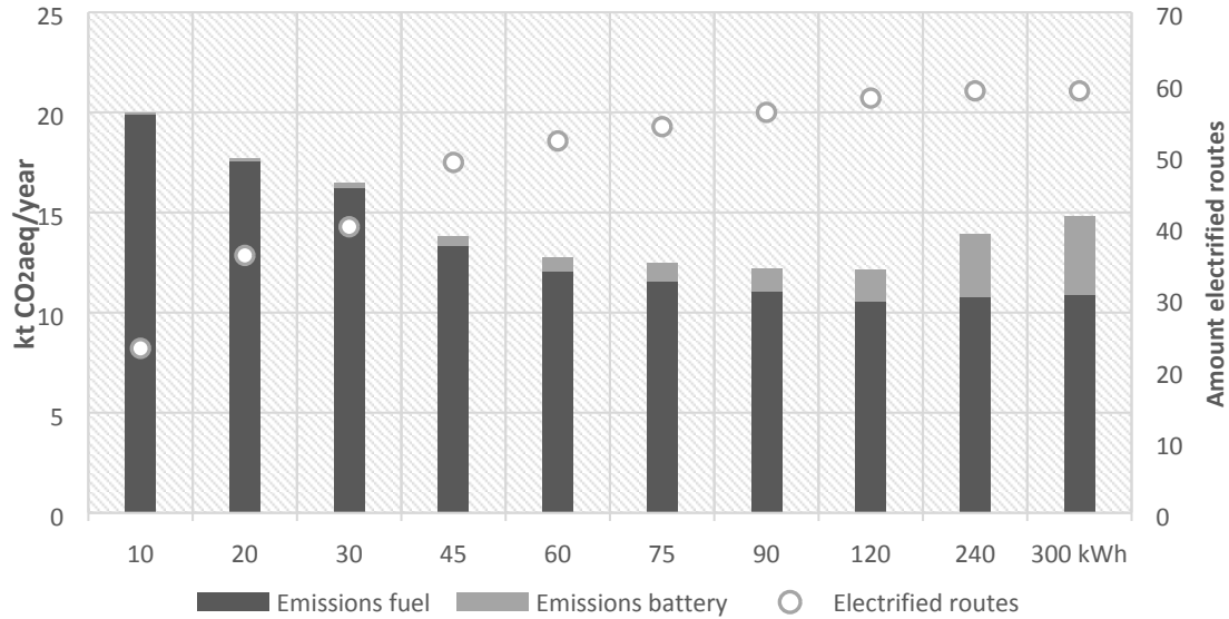
Figure 9: Sensitivity analysis of total emissions in relation to battery capacity, adjusting the energy consumption to the weight of the battery
