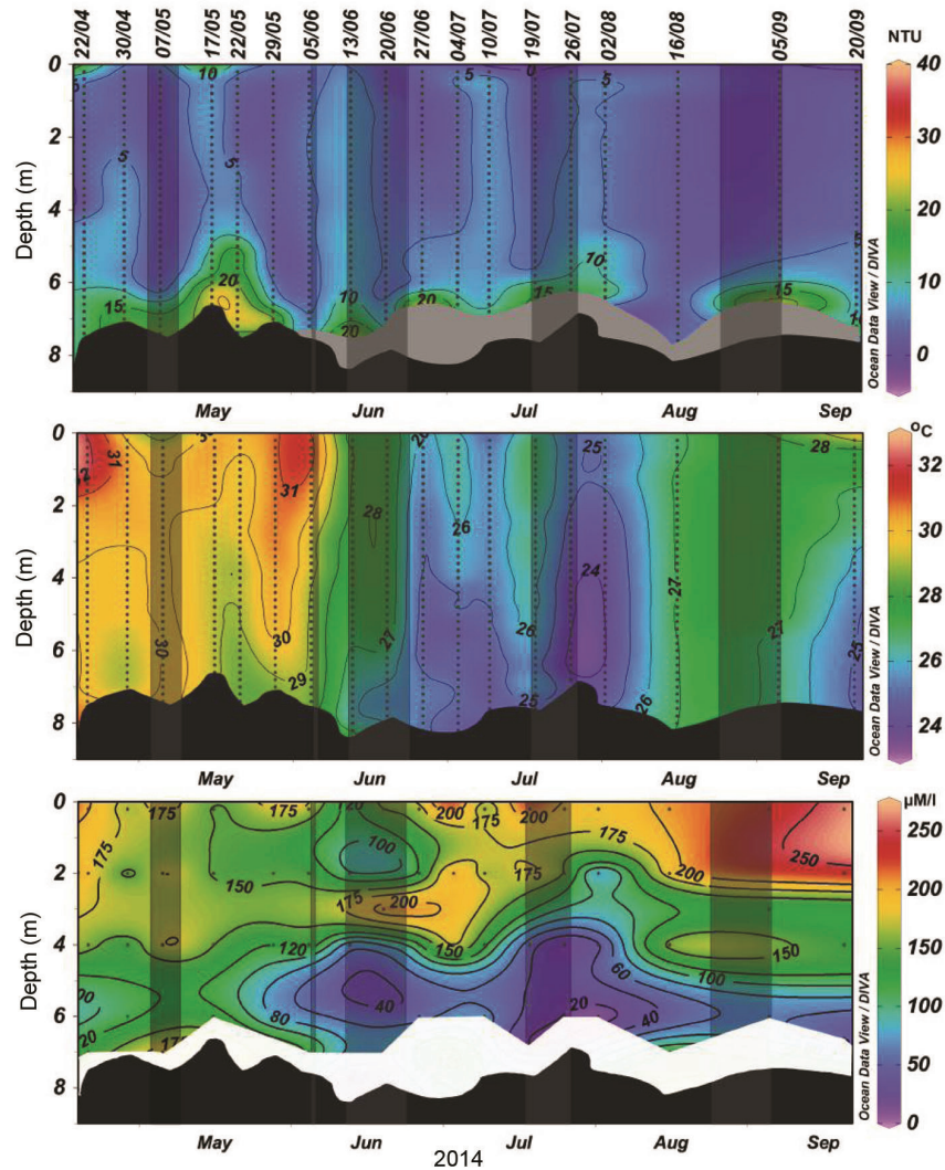
Figure 3. Time-series data on (top panel) water column turbidity (NTU), (middle panel) temperature ( ^{\circ}\text{C} ) and (bottom panel) dissolved oxygen ( \mu\text{M/l} ) during the period 22 April to 30 September 2014. The black shading at the bottom of each panel shows the bottom depth. (Top panel) X -axis labels denote the date on which water column sampling was carried out; the grey shading near the bottom marks the region where turbidity is beyond the upper measuring limit of the turbidity sensor, implying prevalence of fluid mud. (Bottom panel) The white shading indicates missing data.
