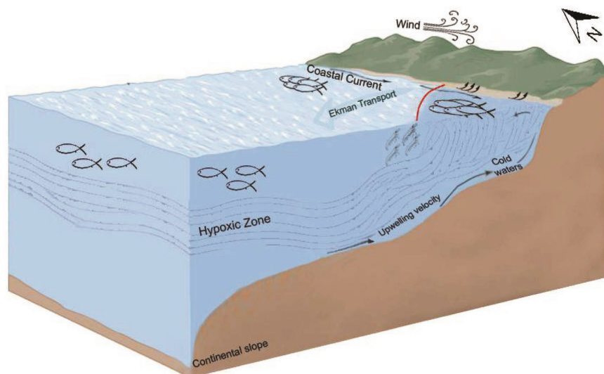
Figure 5. Schematic representation of the coastal upwelling process (bunch of thin lines moving vertically upwards along the coastal region) that co-exists with the mudbank. The semi-circular solid red line indicates the region of mudbank along the coast of Alappuzha. Upwelling brings cold and nutrient-rich water with very low dissolved oxygen from the subsurface to the surface along the coast, making the waters hypoxic. The upwelling-driven phytoplankton bloom sustains the small pelagic fish such as mackerels and sardines during this period. For feeding, these pelagic fish swim against the coastal current which is southerly along the coast, indicated by the solid black arrows close to the coast.
