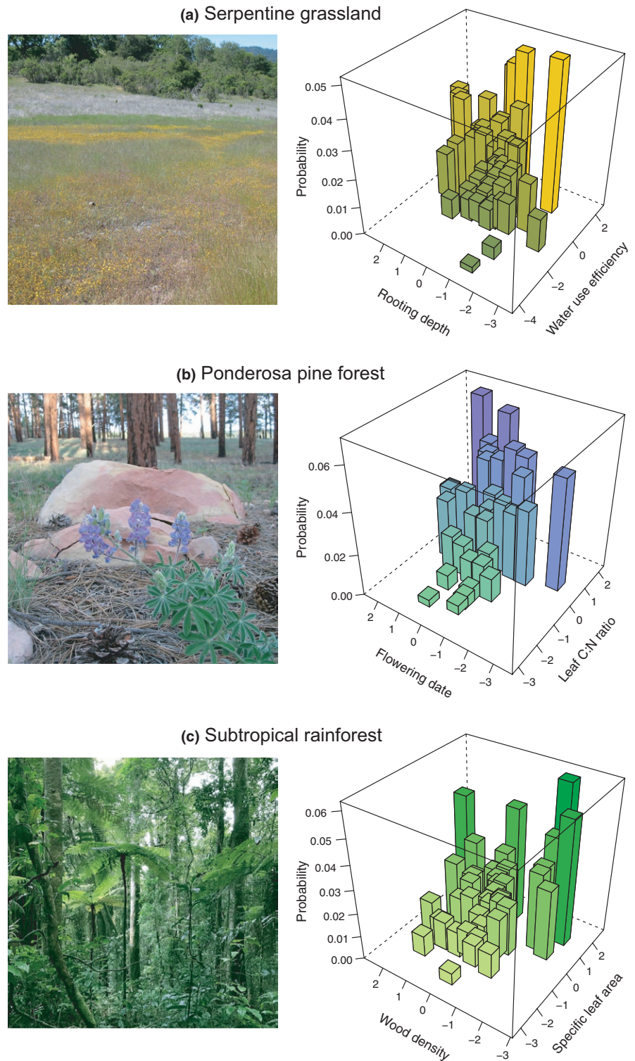
FIGURE 5 Examples of species assemblages (i.e., discrete probability distributions) derived from the selectSpecies R function that simultaneously constrain one trait and diversify another within (a) serpentine grassland in California, USA (photo: J.L. Funk), (b) ponderosa pine forest in Arizona, USA (photo: D.C. Laughlin, and (c) subtropical rainforest in Queensland, Australia (photo: Brandon Clark). Each bar represents one species and its location within the two-dimensional trait space
