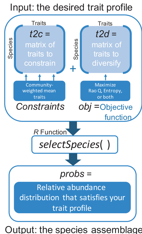
FIGURE 1 The input to selectSpecies() function is a user-specified trait profile of the desired community, which consists of a matrix of traits to constrain (' t2c '), a vector of constraints consisting of community-weighted mean (CWM) traits, a matrix of traits to diversify (' t2d '), or alternatively a distance matrix, and the objective function (' obj ') to maximize (quadratic entropy, entropy, or both). The output of the function (' probs ') is a relative abundance distribution, i.e., proportional abundances for every species in the species pool
