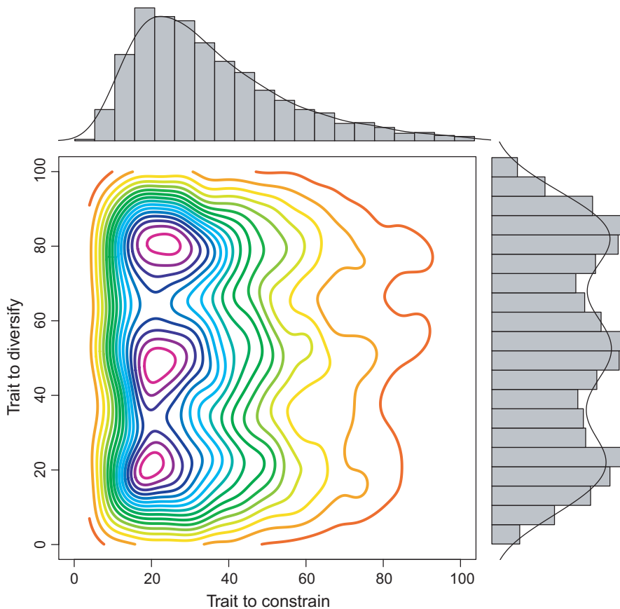
FIGURE 2 Hypothetical community-level trait distribution represented as a bivariate contour density plot, where red = low density and purple = high density. Marginal histograms are also shown for each trait axis. If the goal of the restoration is to re-assemble a community that exhibits convergence toward a specific value of one trait (i.e., the trait to constrain on the x-axis) and diversity of another trait (i.e. the trait to diversify on the y-axis), then the species that are selected for the project must reflect a complex multidimensional trait distribution
