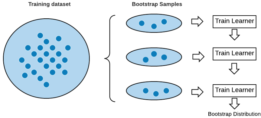
Figure 2.2: Bootstrap Sampling
