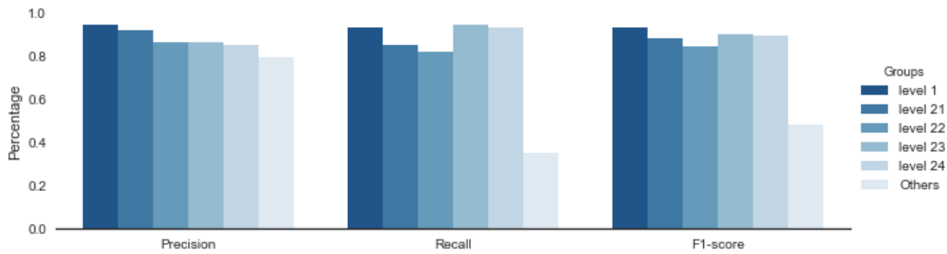
Figure 4.3: Performance of random forest classifier for different groups in case 3
