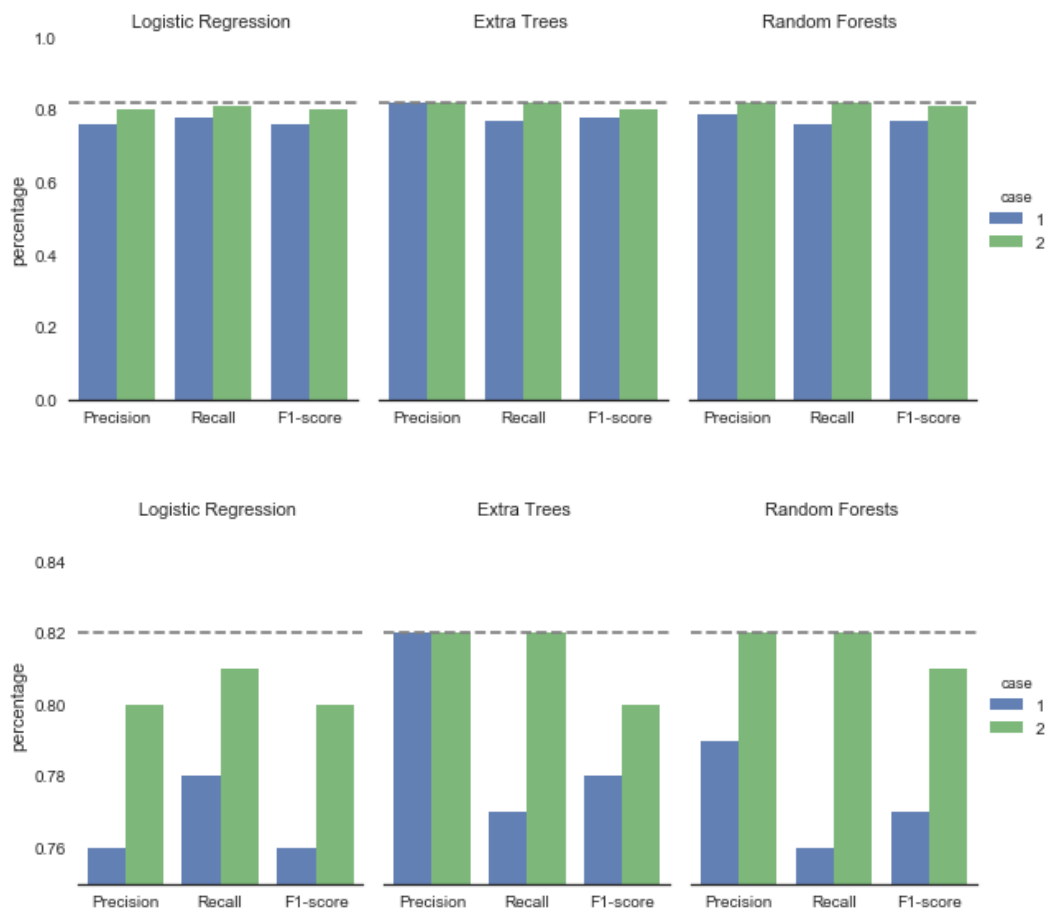
Figure 4.1: Performance comparison of three classifiers in case 1 and 2
