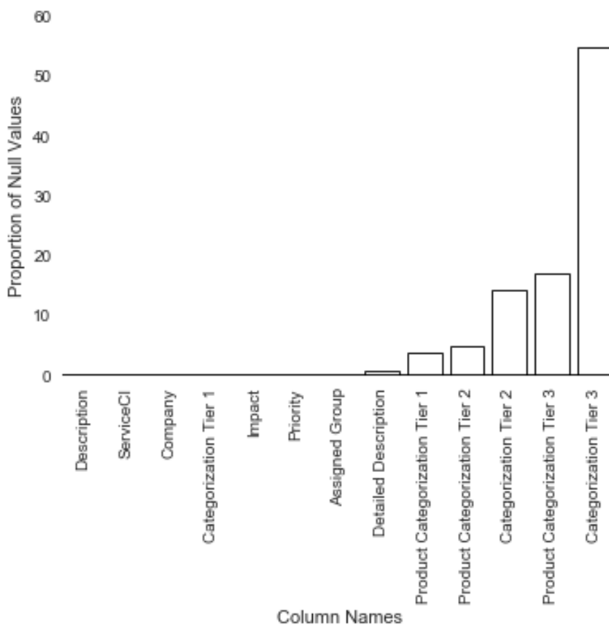
Figure 3.2: Proportion of null values
