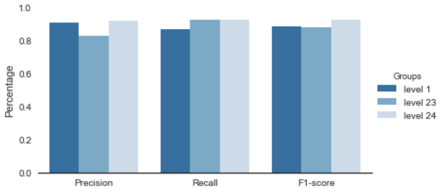
Figure 4.4: Performance of the model in production for level 1, level 23, level 24 groups
