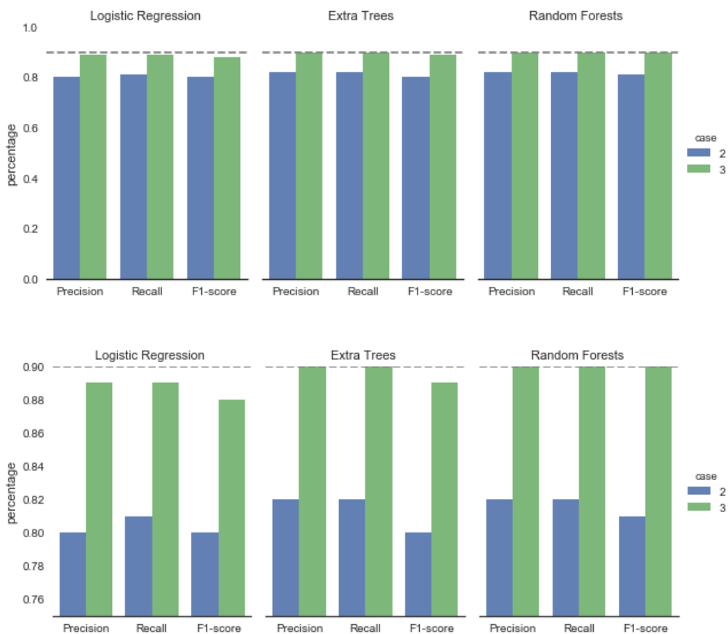
Figure 4.2: Performance comparison of three classifiers in case 2 and 3
