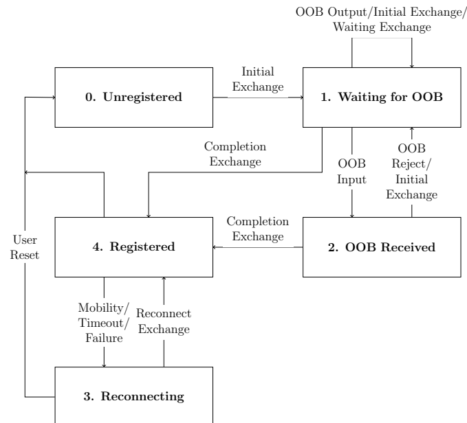
Figure 3.2: EAP-NOOB State Machine [3]
