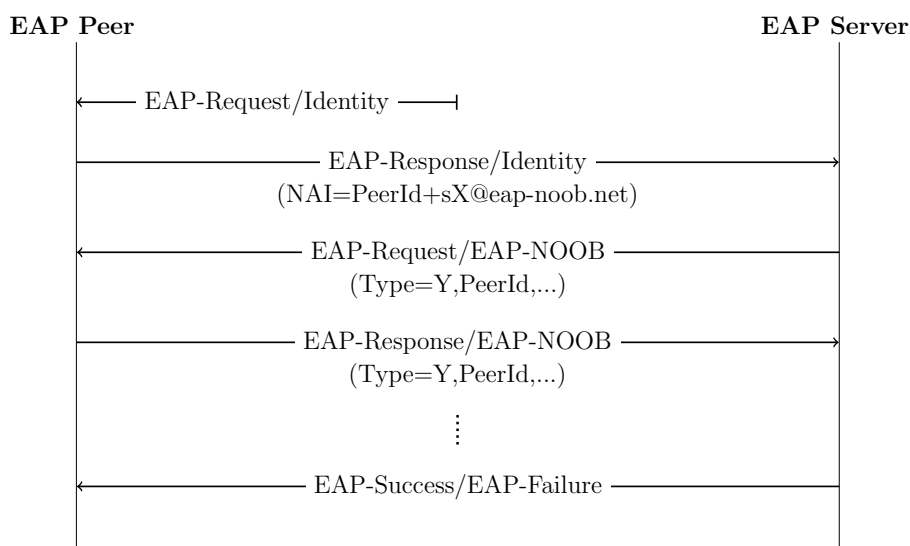
Figure 3.3: EAP-NOOB Exchange
