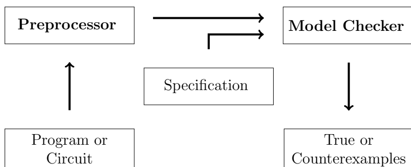
Figure 2.4: Overview of a Model Checker [16]
