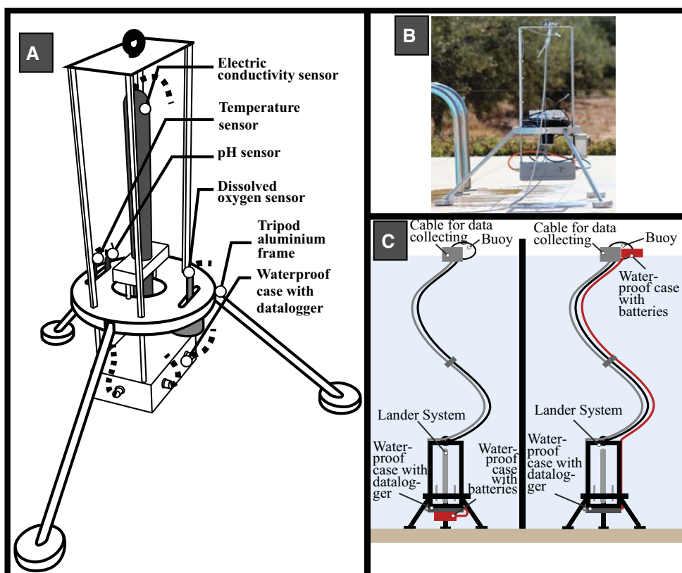
Fig. 2 a Technical sketch of the Lander System with its different components (sensors, tripods aluminium frame, datalogger). b Photograph of the Lander System not equipped with the conductivity sensors. c Two different configuration of the Lander System were used during measurements. On the left, the waterproof case with the batteries is placed directly on the Lander System making necessary to recover it for battery changes. On the right, the waterproof case with the batteries is place on the buoy allowing batteries changes without recovery of the Lander System
