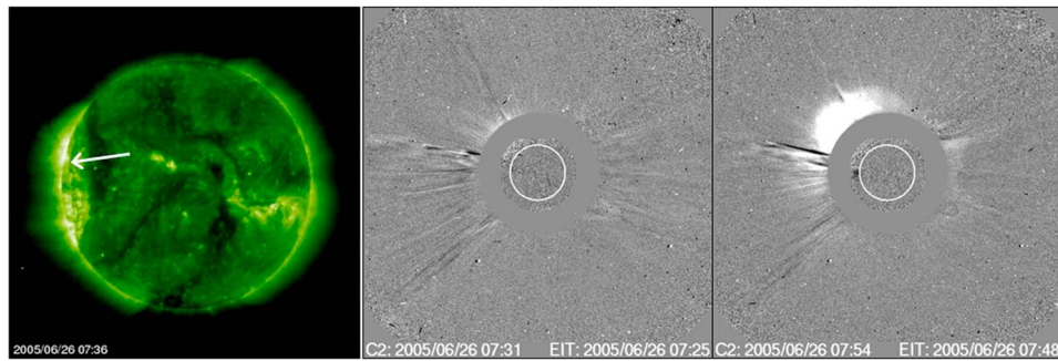
Figure 2. (left) EIT image in 195 Å showing the location of the B05 flare on 26 June 2005 at 07:36 UT. The arrow points to a set of newly faint formed loops that can be seen growing at the eastern limb. (middle and right) Two LASCO C2 images at the time of appearance of the CME in the NNE limb (Figure 2, middle) and as it evolved at 07:54 UT (Figure 2, right).
