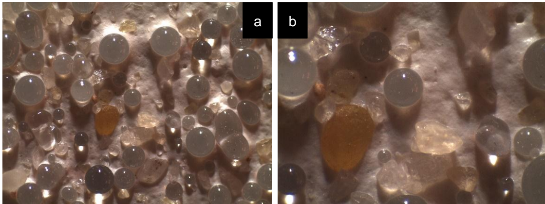
Figure 11. Microscope detail of S9 sample: (a) \times 16 magnifications; (b) \times 35 magnifications.
