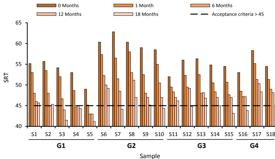
Figure 15. Skid resistance coefficient (SRT) evolution on test samples during the first 18 months of service.
