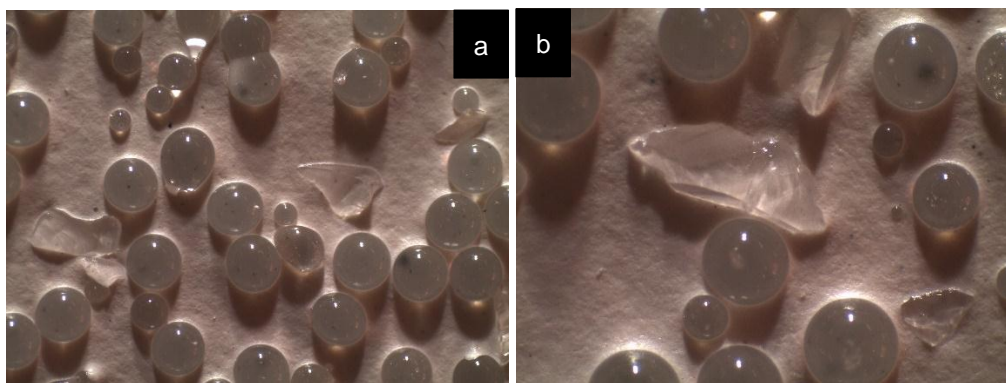
Figure 12. Microscope detail of S15 sample: (a) \times 16 magnifications; (b) \times 35 magnifications.
