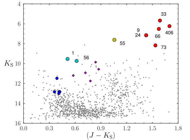
Fig. 6. K_S/(J - K_S) diagram for all stars with good 2MASS data in the field of NGC 3105. Symbols and colours are as in Fig. 5. Stars 9 and 24 occupy the same position in the diagram. Also shown is the location of S406, a likely new cluster RSG not covered by the optical photometry.
