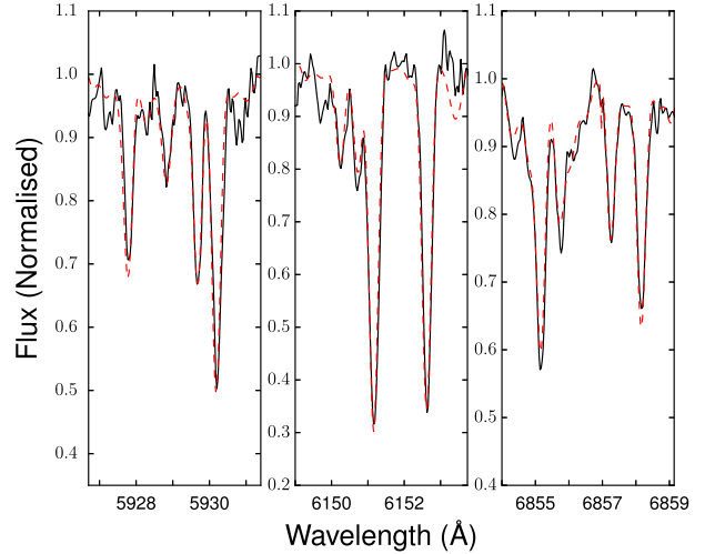
Fig. 10. Some examples of line fits in star 66. Three regions are shown around Fe I \lambda 5927.80 (left), Fe II \lambda 6149.25 (centre), and Fe I \lambda 6855.74 –Fe I \lambda 6858.16 (right). The observed spectrum is the solid black line, whereas the synthetic one is the red dashed line.
