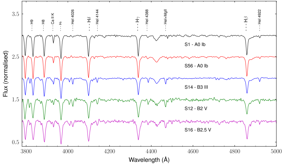
Fig. 2. Spectra of the brightest blue stars in the classical spectral classification region. These spectra have been obtained with grism 14 on EFOSC2. The most important lines are marked.
