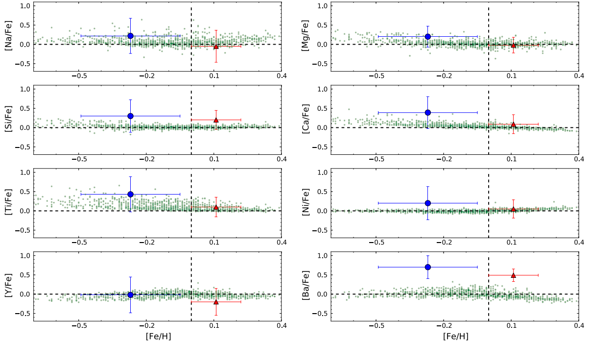
Fig. 13. Abundance ratios [X/Fe] versus [Fe/H] . The green dots represent the galactic trends for the thin disc (Adibekyan et al. 2012; Delgado Mena et al. 2017). NGC 6067 is the red triangle, whereas NGC 3105 (without S24) is the blue circle. Clusters are represented by their mean values. The dashed lines indicate the solar value.
