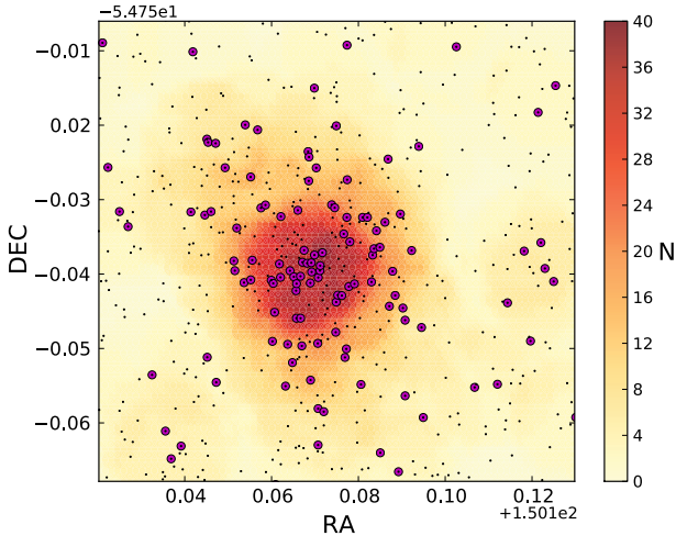
Fig. 9. Sky distribution of the likely members of NGC 3105 (magenta circles) and the rest of the observed stars (black dots) in the field covered by our photometry. Density is computed as the number of stars closer than 0.5 to each point. The overdensity corresponding to the cluster core clearly stands out in the figure.
