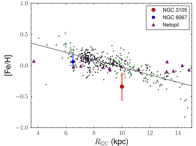
Fig. 12. Iron abundance gradient in the Milky Way found by Genovali et al. (2013, 2014). The black line is the Galactic gradient ( -0.06 dex \text{kpc}^{-1} ), green crosses are Cepheids studied in those papers, whereas black dots show data for other Cepheids from the literature used by these authors. Magenta triangles represent the young open clusters ( <500 Ma) in the sample compiled by Netopil et al. (2016). Finally, the red circle is NGC 3105 and the blue one is NGC 6067. Both young clusters were analysed by our group with the same techniques. NGC 3105 falls well below the metallicity typically observed at its Galactocentric distance. All the values shown in this plot are rescaled to Genovali et al. (2014), i.e. R_{\odot} = 7.95 kpc and A(\text{Fe}) = 7.50 .
