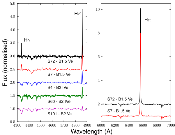
Fig. 3. Spectra of the Be stars in the field of NGC 3105. Left: EFOSC2 spectra around H\beta and H\gamma taken with grism 14 (for stars 4, 7, and 101) and 19 (60 and 72). Right: strong H\alpha emission in stars 7 and 72. These spectra were taken with grating 7 on the SAAO Cassegrain Spectrograph.
