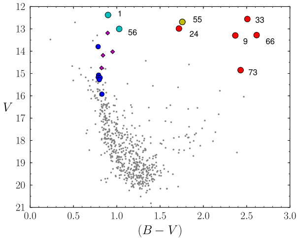
Fig. 5. V/(B - V) diagram for all stars in the field of NGC 3105. Photometric data appear as grey dots. Stars for which we also have spectra are represented by small blue circles (upper main sequence B-type stars), magenta diamonds (Be stars), and filled circles (supergiant stars; colour indicates spectral type: cyan for BSGs, yellow for YSG, and red for RSGs).
