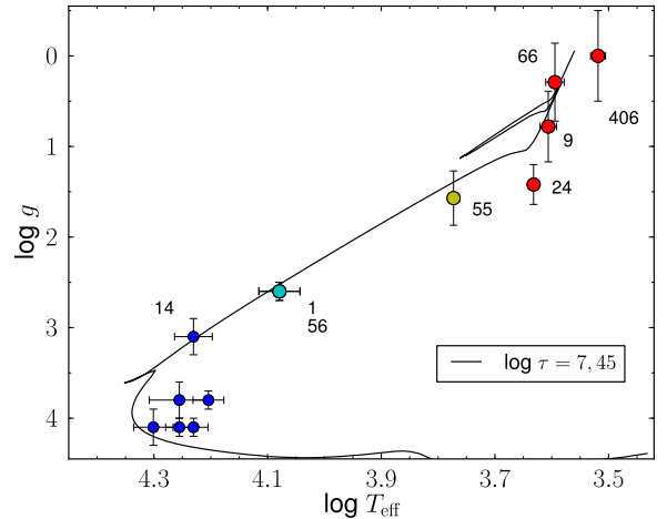
Fig. 11. Kiel diagram for likely members (with the exception of Be stars). Symbols and colours are as in Fig. 5. Stars 1 and 56 occupy the same position on the diagram.
