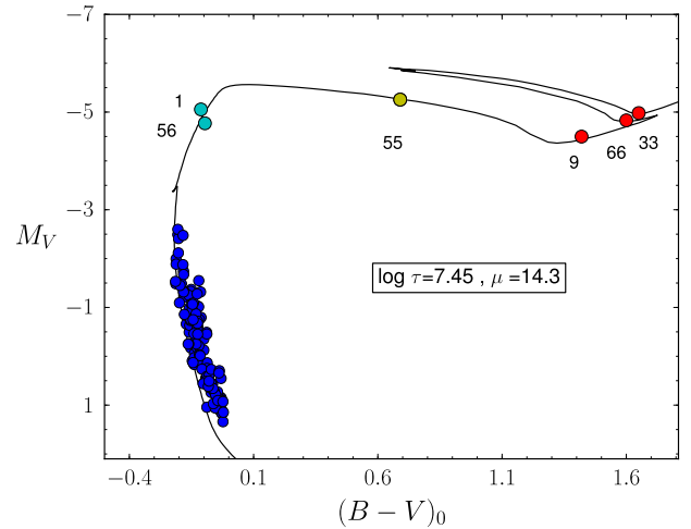
Fig. 8. M_V/(B - V)_0 diagram for likely members of NGC 3105. Symbols and colours are as in Fig. 5. The best-fitting isochrone is the black line.
