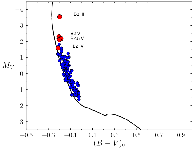
Fig. 7. M_V/(B - V)_0 diagram for likely members of NGC 3105. Stars observed spectroscopically are represented in red. Spectral types for the brightest stars are marked. Blue circles are the rest of the early members found photometrically. The black line shows, as a ZAMS, a PARSEC isochrone of 10 Ma computed at the cluster metallicity. The best-fitting yields a distance modulus of \mu = 14.3 \pm 0.2 .
