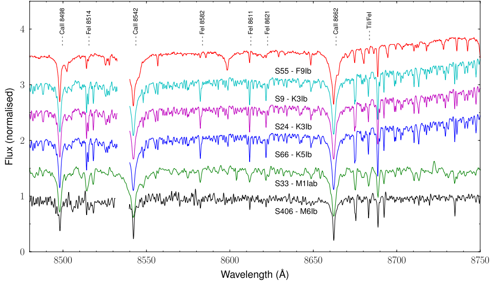
Fig. 4. Spectra of cool supergiant members around the Ca II triplet. All the spectra were taken with FEROS (there is a gap between orders 37 and 38 around 8535 Å), except that of star 33, which was taken with grating 10 on the SAAO Cassegrain Spectrograph.
