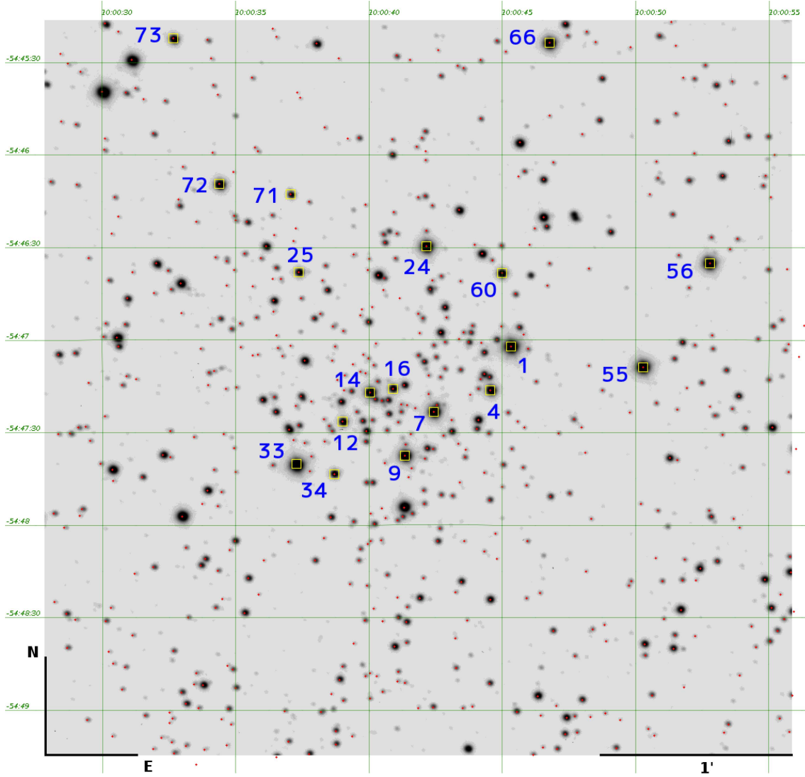
Fig. 1. Finding chart for the 607 stars with photometry in the field of 4.2' \times 4.2' centred on NGC 3105 (red dots). Yellow squares highlight the stars for which we have obtained spectra with the exception of stars 101 and 406, which fall outside the field of view covered by the photometry. The identification of each star corresponds to the WEBDA numbering for this cluster. The image is one of our V -band frames. North is up and east is right.
