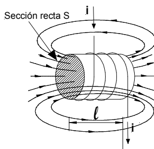
Figura 4 – Bobina recta
