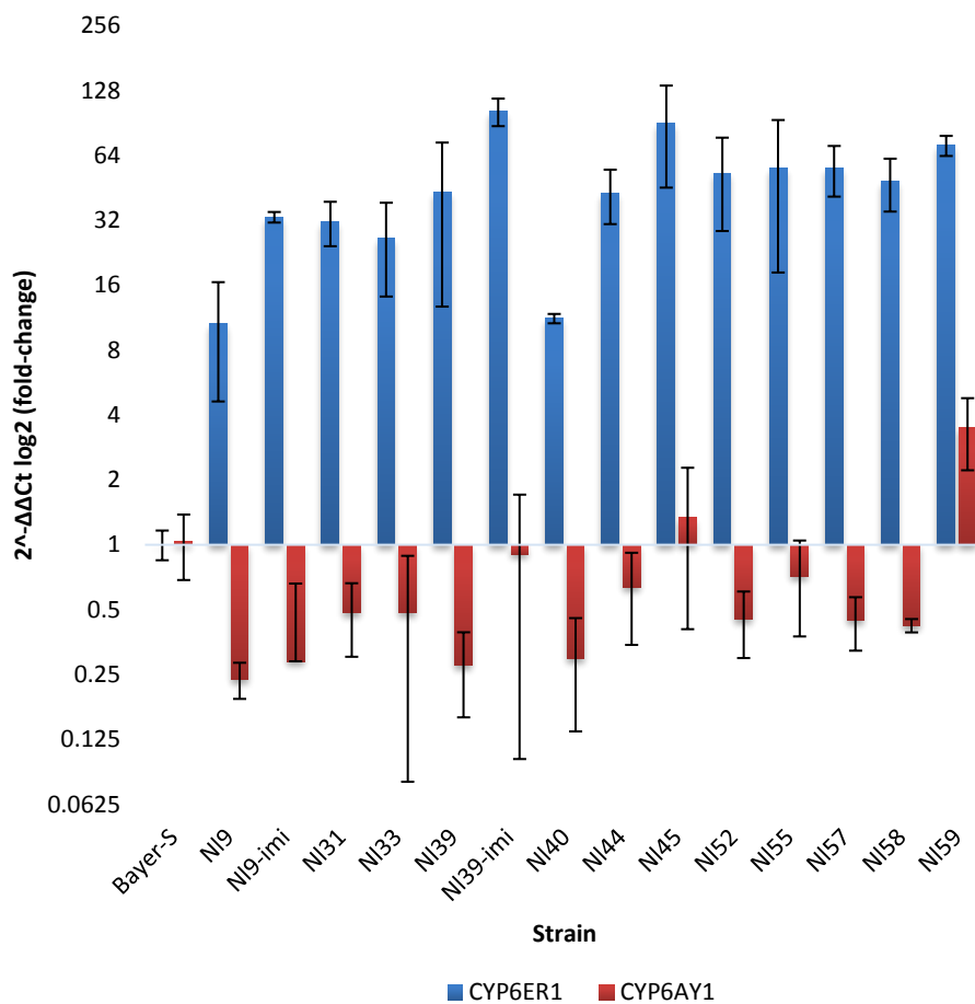
Fig. 6.1 Fold change in expression of CYP6ER1 and CYP6AY1 in 14 resistant N. lugens strains compared with the susceptible reference Bayer-S as determined by qRT-PCR. Error bars display 95% confidence intervals.
