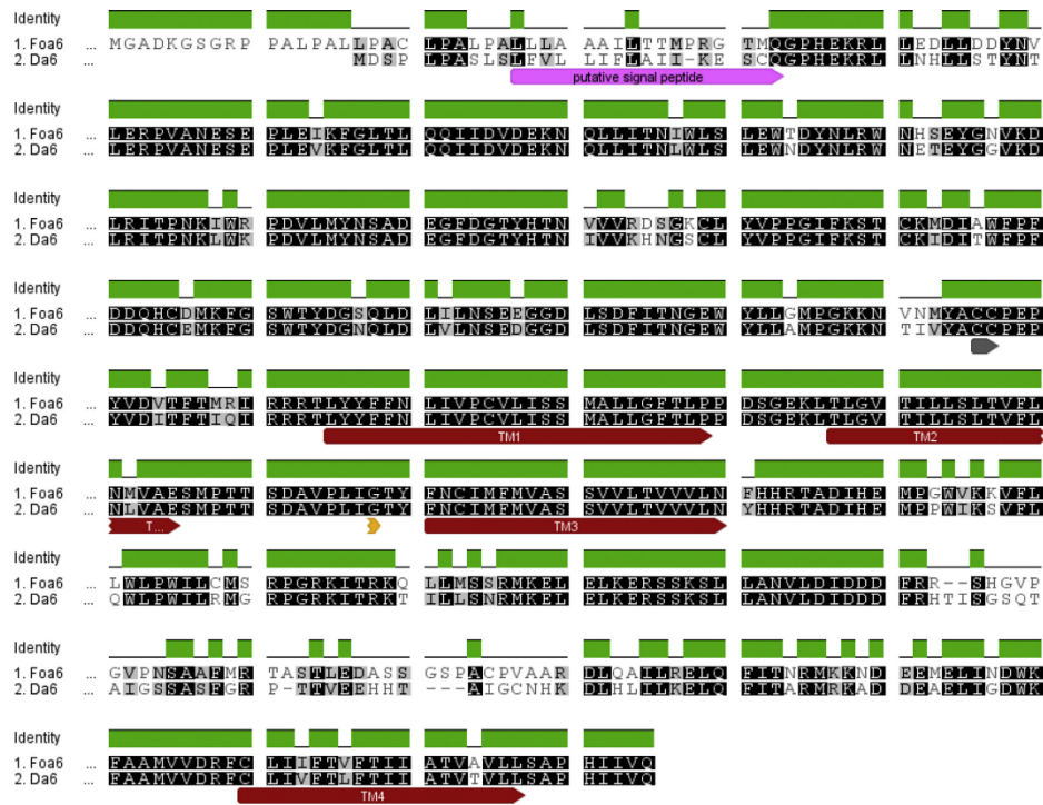
Fig. 5. Amino acid sequence alignment of F. occidentalis nAChR z6 and D. melanogaster nAChR z6 in variant exon 3b/8a. G275E is indicated by an orange arrow and counted from the first amino acid (G) after the putative signal peptide indicated by a pink arrow. Transmembrane regions TM1–4 are annotated with red arrows. (For interpretation of the references to colour in this figure legend, the reader is referred to the web version of this article.)
