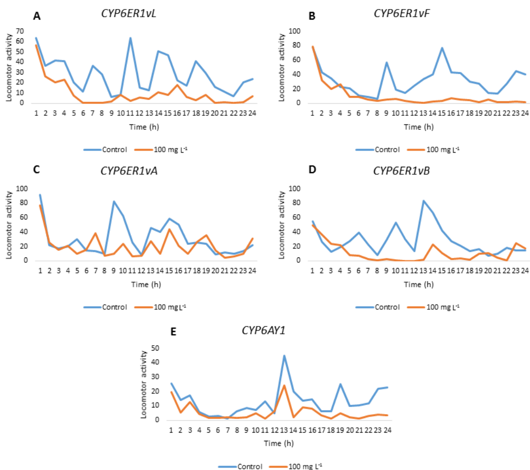
Fig. 6.7 Locomotor activity of CYP6ER1 variants and CYP6AY1 when exposed to 100 mg L -1 imidacloprid. Time displays the number of hours the flies have been on the imidacloprid treated food. Locomotor activity displayed is the average movement recorded for each of the 5 min sections within a given hour.
