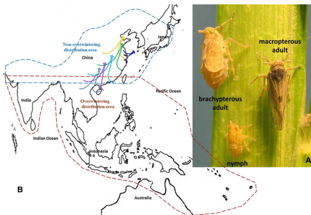
Fig. 1.2 A) A nymph of N. lugens and the short winged (brachypterous) and long winged (macropterous) female adults. B) A map highlighting the overwintering and non-overwintering areas for N. lugens , and possible migration routes of N. lugens from tropics to temperate regions.
