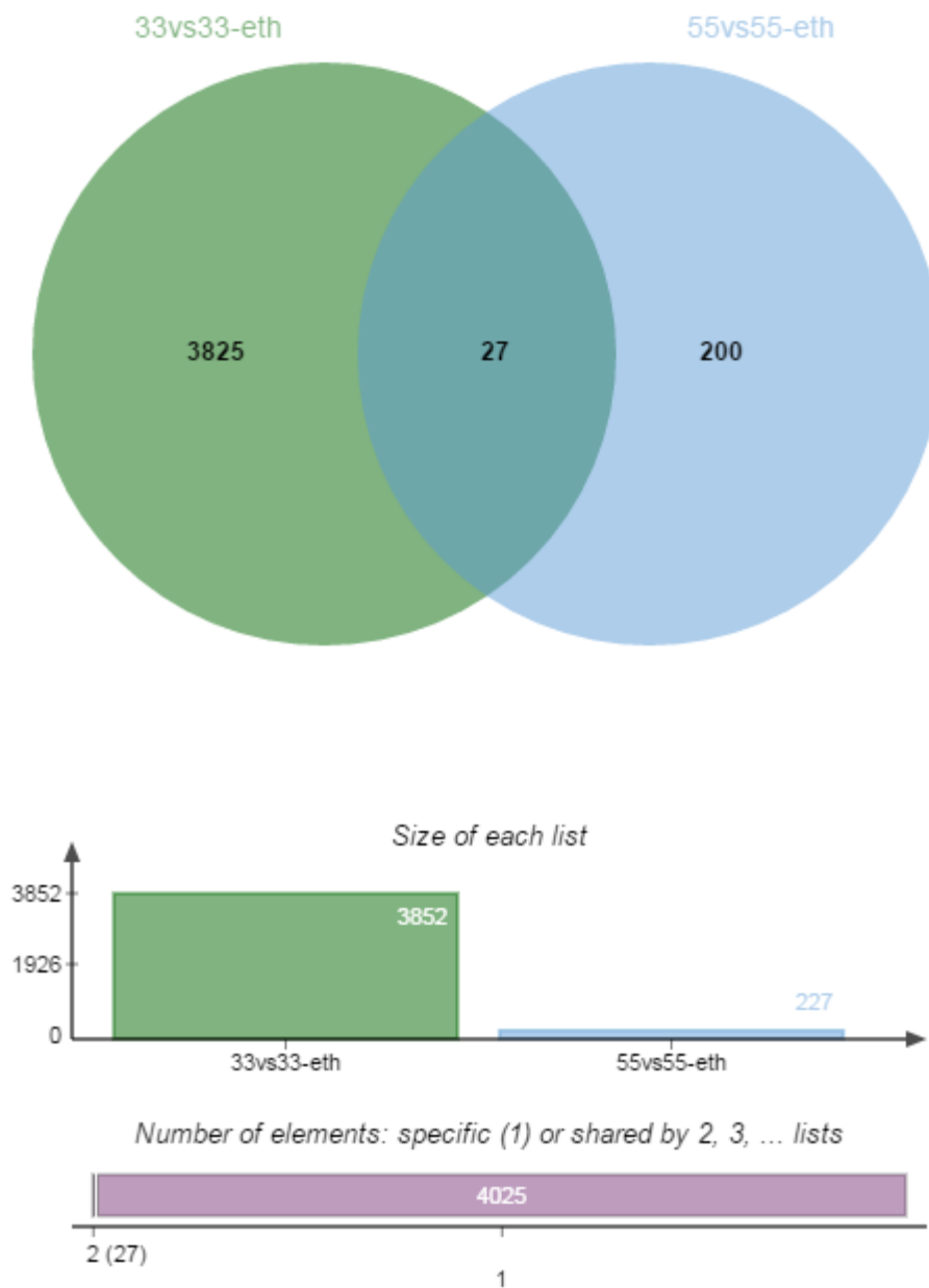
Fig. 4.4 Top: Venn diagram showing differentially expressed transcripts in RNA-Seq between unselected and selected populations of N. lugens . Bottom: differentially expressed transcripts in each comparison.
