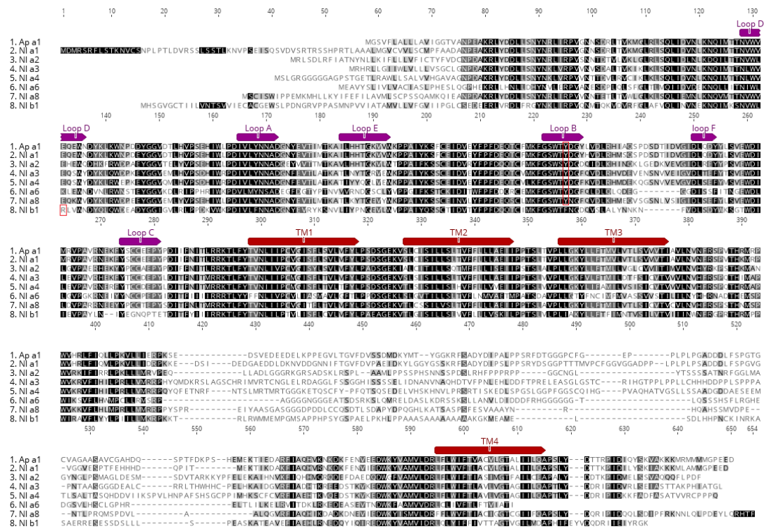
Fig. 4.5 Amino acid sequence alignment of N. lugens nAChR subunits found with the transcriptome. The P. americana \alpha 1 subunit is also displayed. The loop domains are indicated (A-F) by purple bars above the sequence. The transmembrane regions are highlighted by red bars above the sequence. Known mutations involved in neonicotinoid resistance (R81T, Y151S) are boxed in red.
