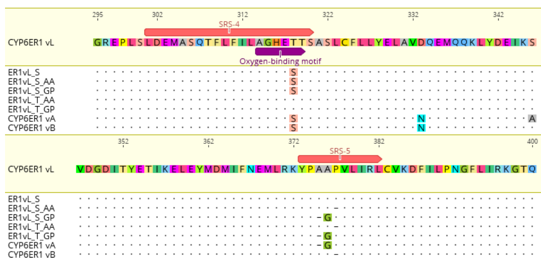
Fig. 6.9 Amino acid alignment highlighting the mutant constructs created with the mutations introduced to CYP6ER1vL .
