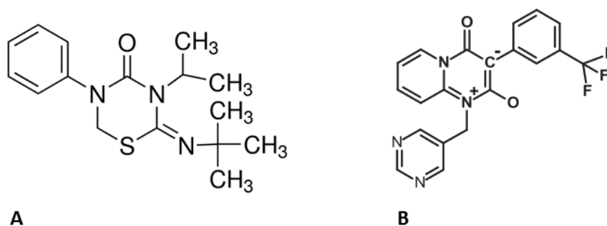
Fig. 1.8 Chemical structures of A) Buprofezin. B) Triflumezopyrim.
