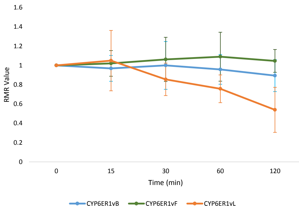
Fig. 6.6 Response curves for CYP6ER1vB , CYP6ER1vF and CYP6ER1vL after treatment with 24 \text{ mg L}^{-1} imidacloprid. Points represent mean RMR values with 95% confidence intervals.
