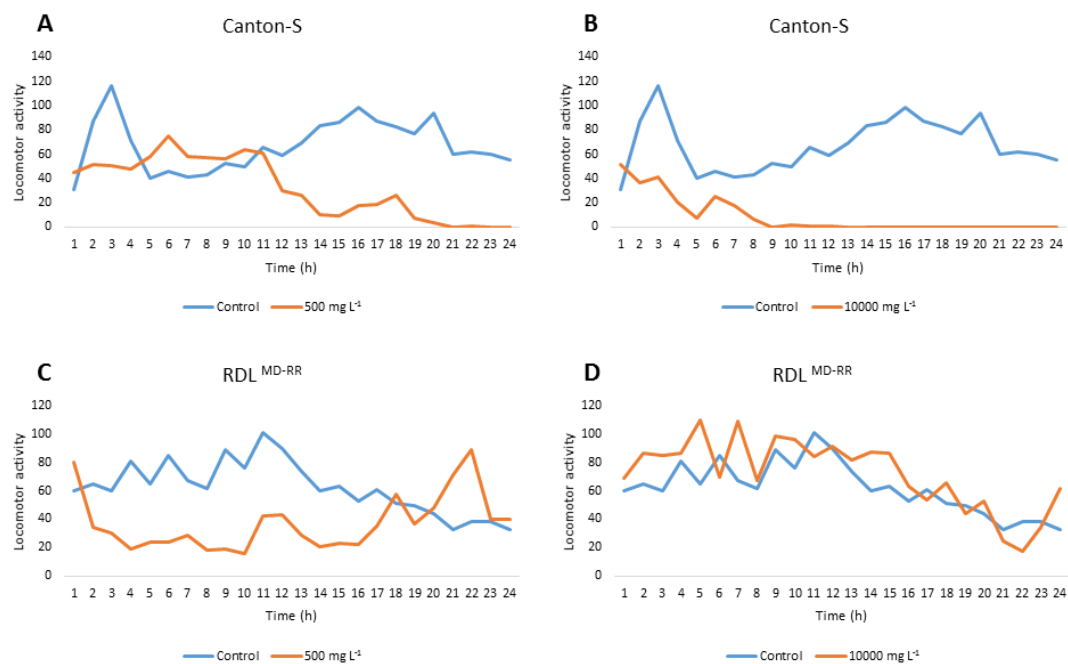
Fig. 5.5 Locomotor activity of Canton-S and RDL MD-RR . A) Canton-S treated with 500 mg L -1 ethiprole. B) Canton-S treated with 10000 mg L -1 ethiprole. C) RDL MD-RR treated with 500 mg L -1 ethiprole. D) RDL MD-RR treated with 10000 mg L -1 ethiprole. Time axis displays the number of hours the flies have been on the ethiprole coated food. Locomotor activity displayed is the average movement recorded for each of the 5 min sections within a given hour.
