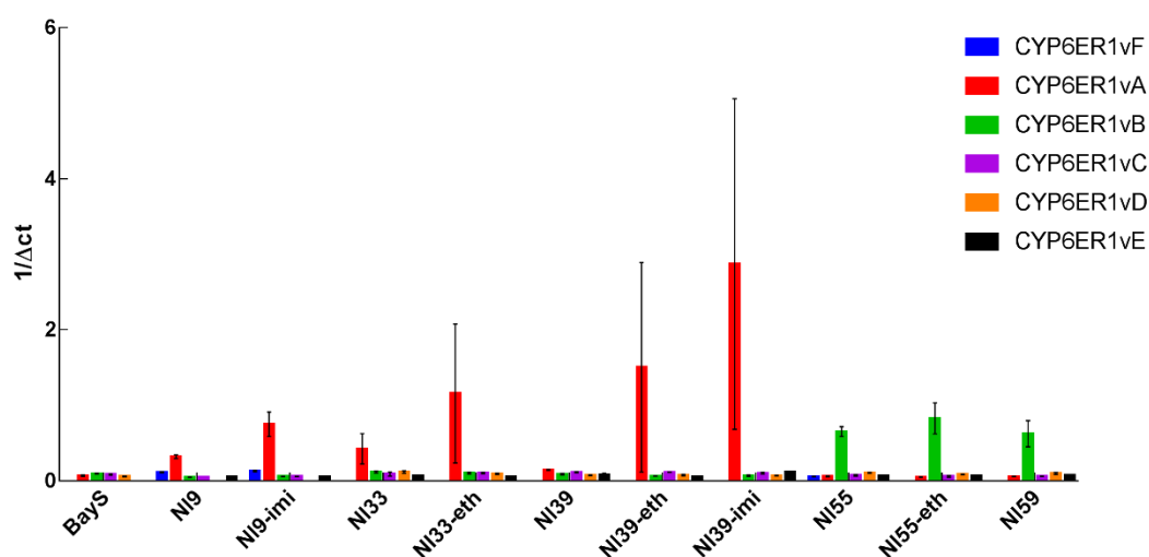
Fig. 6.3 1/\Delta C_t values of CYP6ER1 variants in ten imidacloprid and ethiprole resistant strains and the laboratory susceptible as determined by qRT-PCR.
