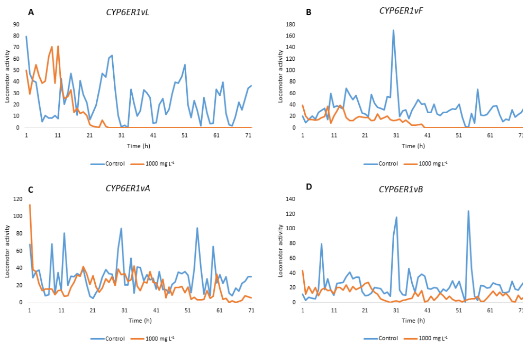
Fig. 6.8 Locomotor activity of CYP6ER1 variants when exposed to 1000 mg L -1 ethiprole. Time displays the number of hours that the flies have been on the ethiprole coated food. Locomotor activity displayed is the average movement recorded for each of the 5 min sections within a given hour.
