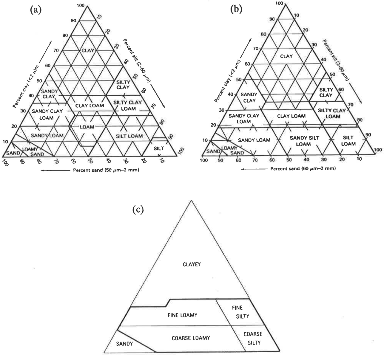
Fig. 2. Textural (particle size) classes according to (a) United States Department of Agriculture; (b) Soil Survey of England and Wales (now Soil Survey and Land Research Centre); and (c) groupings from (b) used to differentiate soil series in England and Wales.
