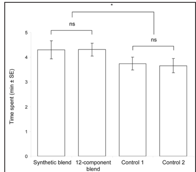
Figure 3. Behavioral response of winged virginoparae Aphis fabae to synthetic blend and twelve-component blend when both odor sources present together in the same olfactometer. * Significantly different ( p < 0.05 ).
