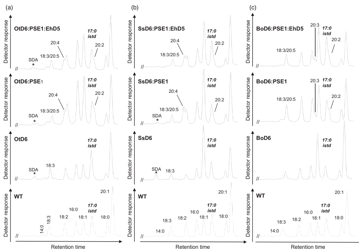
Figure 4 Acyl-CoA profiles of transgenic Arabidopsis. Acyl-CoA profiles of developing seeds of wild type (wt) and single-, double- and triple-transgenic Arabidopsis lines, expressing OtD6 (a), SsD6 (b) and BoD6 (c). The internal standard ( I std ) is 17:0 acyl-CoA. The positions of transgene-derived non-native fatty acids are indicated.
