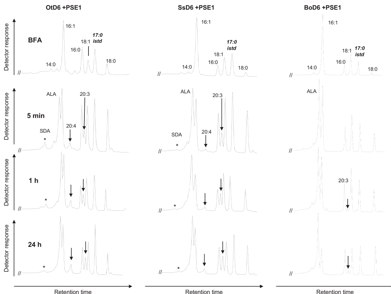
Figure 2 Kinetic analysis of fatty acid changes in acyl-CoAs of yeast co-expressing \Delta 6 -desaturases and PSE1. Cultures of yeast co-transformed with one of the \Delta 6 -desaturases (OtD6, SsD6 or BoD6) and PSE1 were grown for 24 h at 30 °C in the presence of galactose before being supplemented with 250 \mu\text{M} \alpha -linolenic acid (ALA). The acyl-CoA pool composition of the transgenic yeast was analyzed before adding ALA (BFA) and as well as 5 min, 1 and 24 h after substrate was supplied to the medium. The desaturated product stearidonic acid (SDA) is marked by a star, and elongated products are indicated with arrows. Data shown are representative for three independent experiments. The internal standard ( I_{std} ) is 17:0 acyl-CoA.
