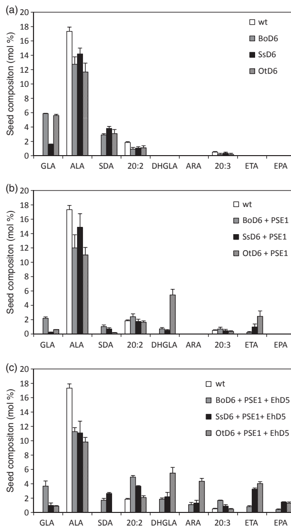
Figure 3 Total fatty acid composition of seeds from transgenic Arabidopsis lines. FAMES were analyzed from wild type (wt), single-transgenic lines expressing \Delta 6 -desaturases (a), double-transgenic lines co-expressing \Delta 6 -desaturases and PSE1 (b) and triple-transgenic lines of Arabidopsis, co-expressing \Delta 6 -desaturases, PSE1 and EhD5 (c). Each value represents the mean \pm SD of 10 independent lines. In all cases, the SD was <1.
