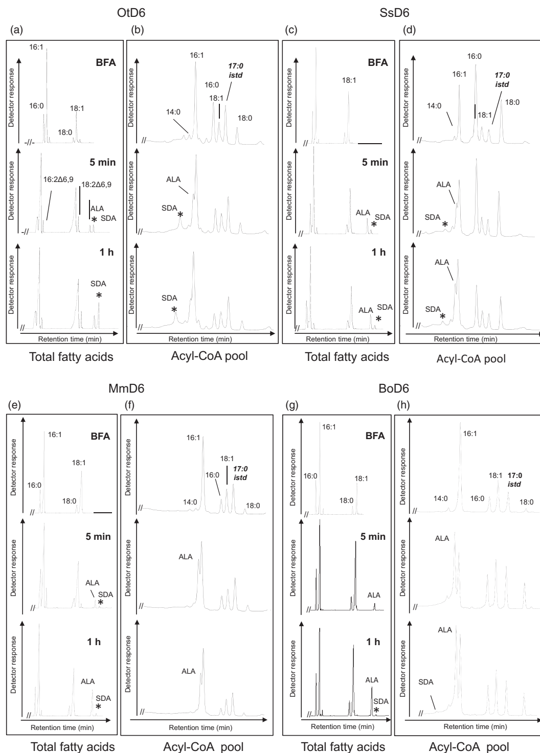
Figure 1 Kinetic analysis of fatty acid profiles in lipids and acyl-CoAs of yeast expressing \Delta 6 -desaturases in the presence of \alpha -linolenic acid (ALA). Cultures of yeast transformed with OtD6, SsD6, MmD6 and BoD6 were grown for 24 h at 30 °C in the presence of galactose before being supplemented with 250 \mu M ALA. The fatty acid composition as well as the acyl-CoA pool composition of the transgenic yeast was analyzed before adding ALA (BFA = before addition) as well as 5 min and 1 h after substrate was supplied to the medium. The desaturated product stearidonic acid (SDA) is marked by a star. Data shown are representative for three independent experiments, with chromatographic resolution occurring against time (X-axis). Detector response (Y-axis) is derived from FID (a) or FLD with the excitation wavelength was set to 230 nm and the emission wavelength to 420 nm. (a) Fatty acid composition of yeast cells expressing OtD6 (a, b), SsD6 (c, d), MmD6 (e, f) and BoD6 (g, h) in the presence of ALA. (b) Acyl-CoA profiling of yeast cells expressing OtD6, MmD6, SsD6 and BoD6 in the presence of ALA. The internal standard ( I_{std} ) is 17:0 acyl-CoA.
