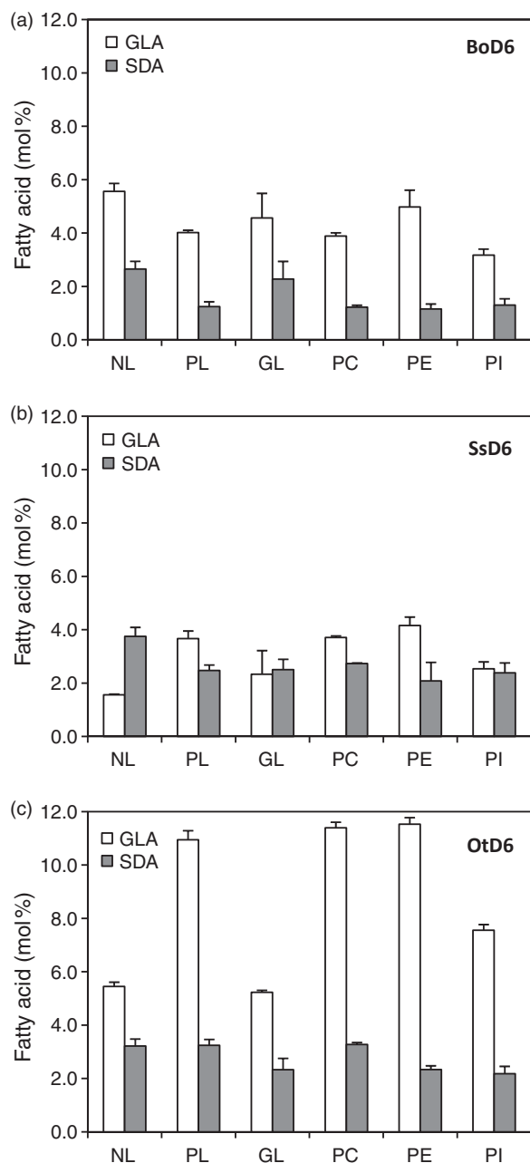
Figure 5 Distribution of GLA and stearidonic acid (SDA) within the different lipid fractions of transgenic Arabidopsis seeds, expressing different \Delta 6 -desaturases (a, BoD6; b, SsD6; c, Otd6). Mature Arabidopsis seeds were used for lipid analysis. The ratios were calculated as (products/educt) using values corresponding to per cent of total fatty acids. The values are the mean \pm SD (<1) of three independent lines.
