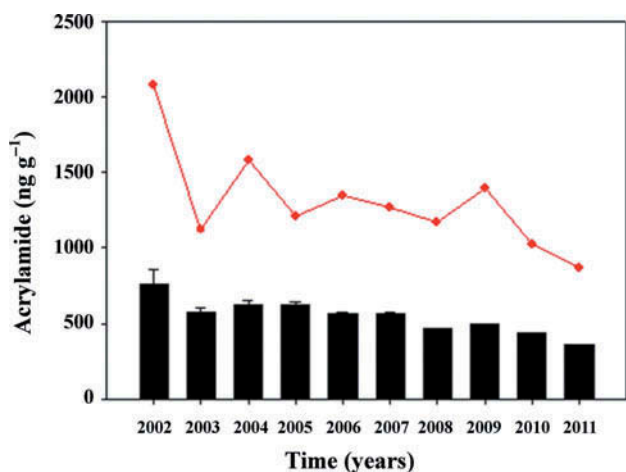
Figure 2. Overall mean acrylamide levels ( \text{ng g}^{-1} ) in samples of potato crisps shown over years from 2002 to 2011, with standard errors and with trend in 95% (Q95) quantiles (red).
