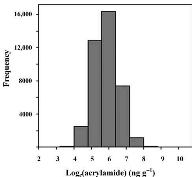
Figure 1. Distribution (histogram) of the \log_e(\text{acrylamide}) values ( \text{ng g}^{-1} ) in samples of potato crisps.
