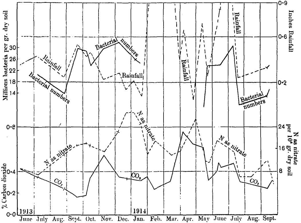
Fig. 14. Curves showing rainfall, bacterial numbers in soil, CO 2 in soil air and nitrate in soil of Broadbalk dunged plot.
