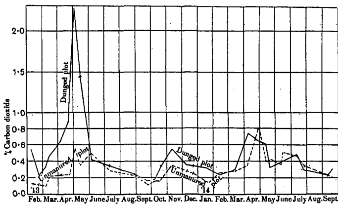
Fig. 10. Comparison of CO 2 content of unmanured plot with plot receiving farmyard manure, Broadbalk field.
