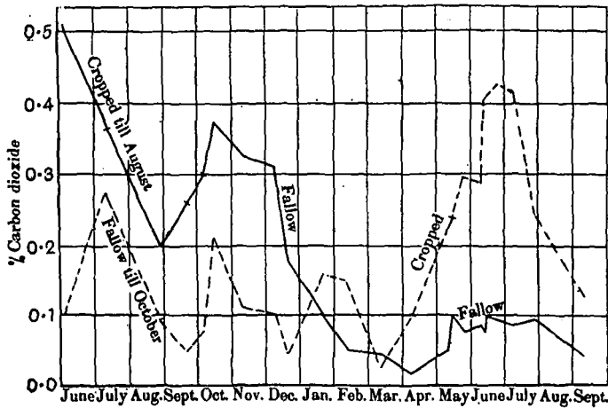
Fig. 11. Curves showing percentage of CO 2 in air of Hoos wheat and fallow plots.
