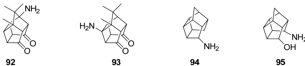
Figure 29. Derivatives of pentacyclo[5.4.0.0 2,6 .0 3,10 .0 5,9 ]undecane.
