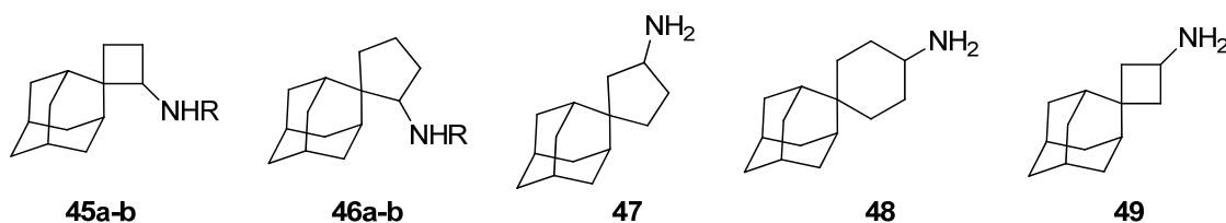
Figure 19. Aminospiroadamantanes 45-48 and unknown compound 49 . a, R = H; b, R = methyl.
