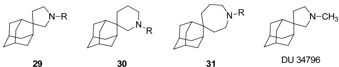
Figure 13. Spiro adamantane derivatives synthesized by N. V. Philips-Duphar. R is a lower alkyl group.
