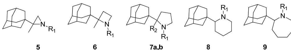
Figure 6. Heterocyclic rimantadine analogs.
