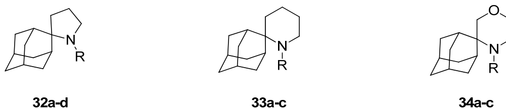
Figure 14. Azaspiro- and oxazaspiro-adamantane derivatives. a, R = H; b, R = methyl; c, R = ethyl; d, R = cyclopropylmethyl.
