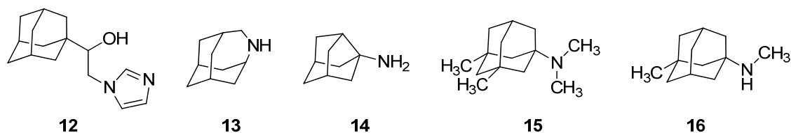
Figure 8. Some of the amantadine analogs reported by Scholtissek and coworkers.
