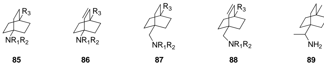
Figure 27. Bicyclo[2.2.2]octan-1-amine, 85 , and related compounds.
