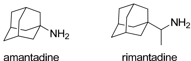
Figure 1. The structures of the anti-influenza A drugs amantadine and rimantadine.
