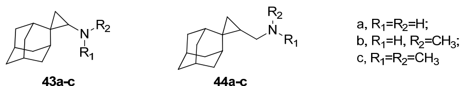
Figure 18. Aminospiroadamantanes 43 and 44 .
