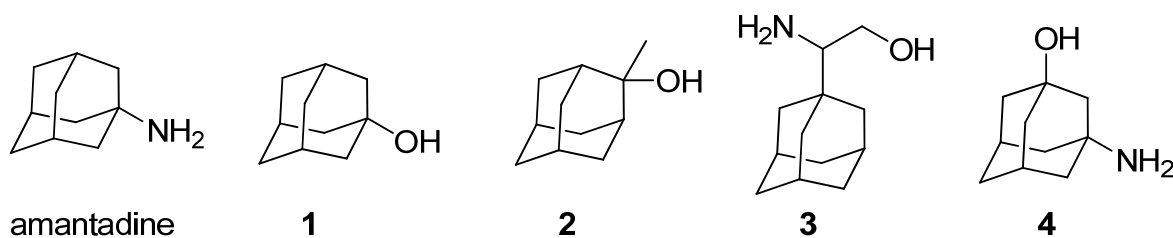
Figure 5. Several hydroxylated analogs of amantadine. IC_{50} values (against wt M2 channel): amantadine ( 16 \mu M ), 1 ( 20 \mu M ), 2 ( 14 \mu M ), 3 ( 16 \mu M ), 4 (not active).
