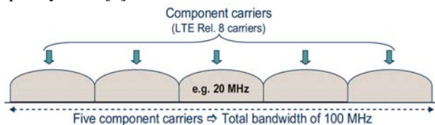
Fig. 1, Carrier Aggregation
