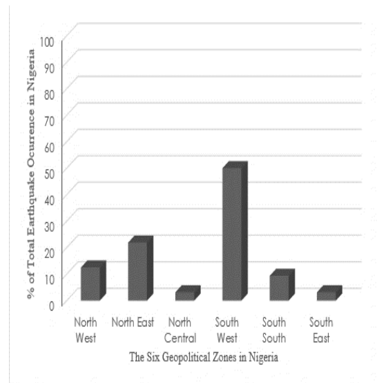
Fig.1 Regionalization of Nigeria Seismicity
