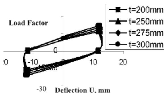
Fig. 3 Hysteresis curve with stiffness decay
