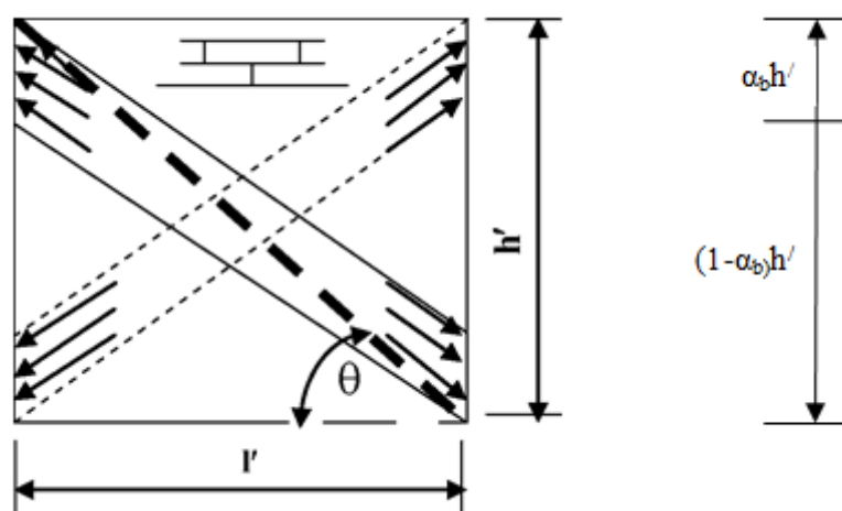
Figure 2 (b) Straw bale wall infill panel wall equivalent diagonal strut
