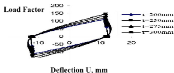
Figure 4 Hysteresis curve with strength degradation
