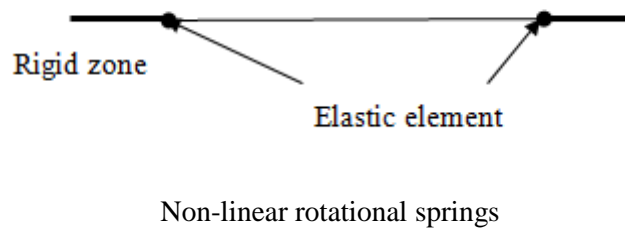
Figure 1 One-dimensional model for beam and column
