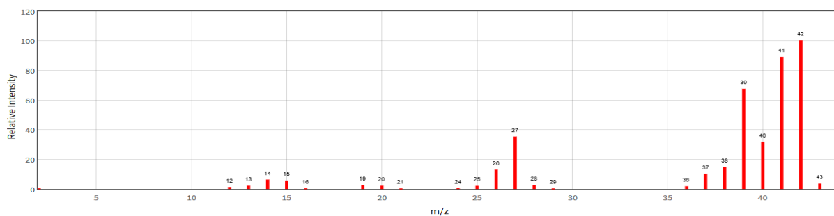
FIG. 4: CYCLOPROPANE MASS SPECTRUM
