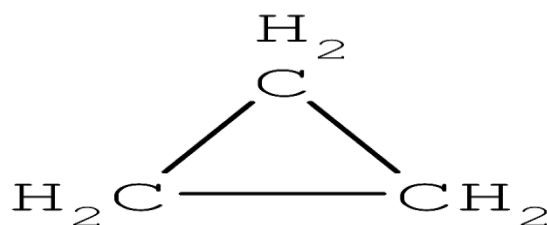
FIG. 3: STRUCTURE OF CYCLOPROPANE
