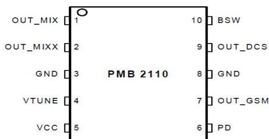
Fig 3: PIN Configuration of the PMB 2110 VCO
