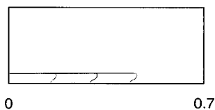
FIG. 7. Phase field model simulation of the spontaneous nucleation in CCH5. One-quarter of the nematic–smectic- B interface is represented using \Delta=0.16 , 300\times 300 grid points, \Delta x=\epsilon=0.005 , \beta=350 , n=20 , and \Delta t=8\times 10^{-6} . The times corresponding to the different contours of the interface are t=0.035 , 0.070 , 0.105 .
