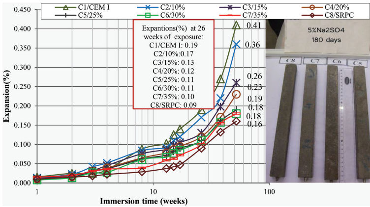
Figure 12. Length changes over time of prismatic mortars immersed in 5% Na 2 SO 4 [5].
