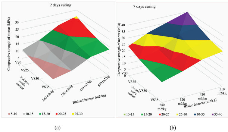
Figure 3. Effect of fineness on compressive strength of VS-based cement mortars cured for 2 (a) and 7 (b) days [89].
