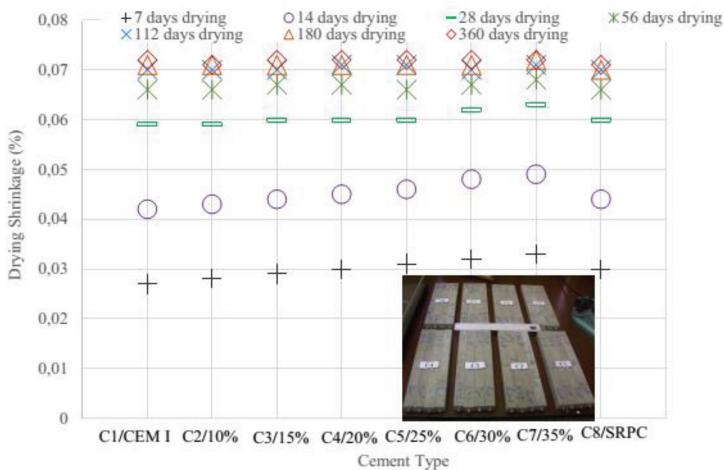
Figure 11. Drying shrinkage values of prismatic mortar specimens [99].
