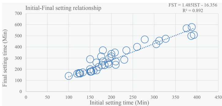
Figure 4. Relationship between initial and final setting times.
