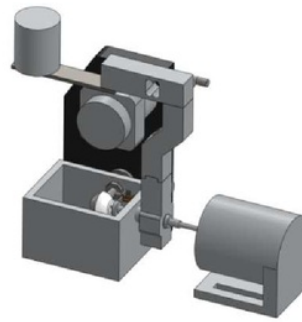
Figure 8. Optimal Design of Tribometer
