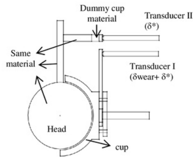
Figure 4. Displacement Transducer Mechanism
