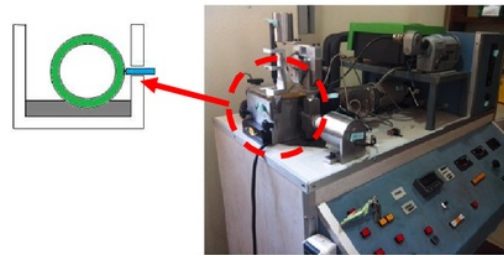
Figure 1. Pin-on-ring Tribometer
