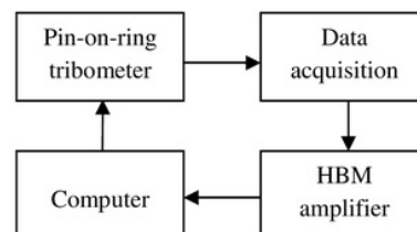
Figure 2. Work Schematic of Pin-on-Ring Tribometer
