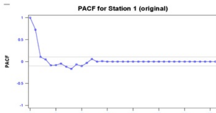
Gambar 6. Plot PACF data inflow
