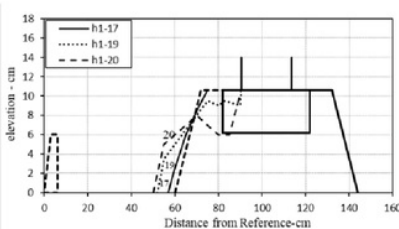
Fig.13. The scouring profile of the T structure modeling at L_2
