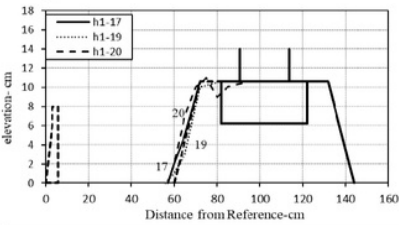
Fig.14. The scouring profile of the T1 structure modeling at L_2
