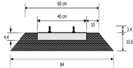
Fig.2. The section of the ballast model
