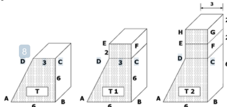
Fig.5. The T, T1, and T2 type of external prevention structures (in centimeter)
