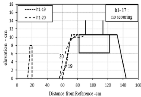
Fig.10. The scouring profile of the T1 structure modeling at L 1
