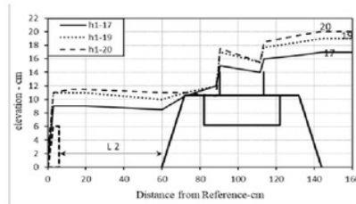
Fig.12. The water level variation of the T structure modeling at L_2
