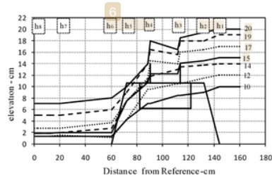
Fig.6. The profiles of various water levels simulated without prevention structure ( h_1 = 10-20 cm)
