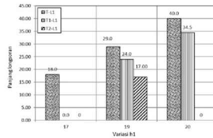
Fig.16. The scouring length structure at L1
