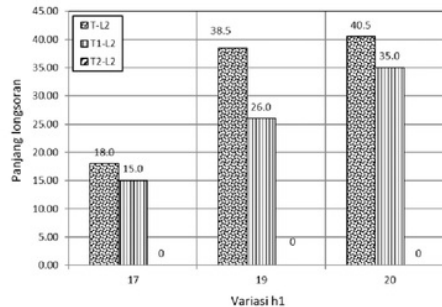
Fig.17. The scouring length structure at L2
