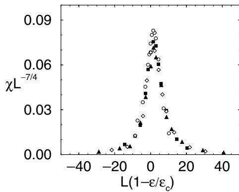
FIG. 4. Finite-size scaling function of the susceptibility \chi with the 2D-Ising critical exponents.
