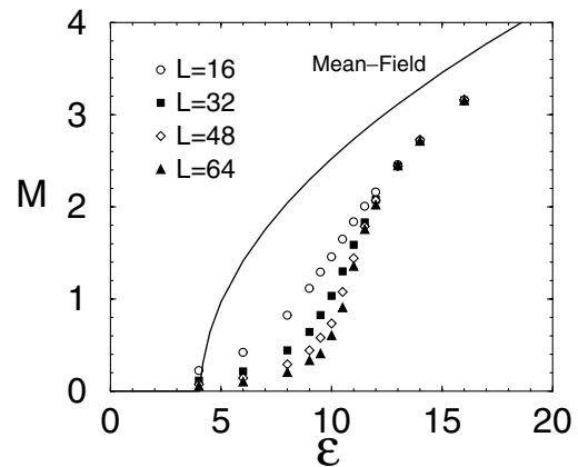
FIG. 1. Inverted phase diagram: intensive order parameter M as a function of the noise intensity for a = 1 , c = 0.5 , K = 1 , and for four different system sizes. The continuous line is the Weiss mean-field result.
