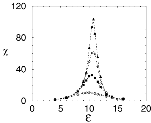
FIG. 2. Generalized susceptibility \chi versus noise intensity for the case of Fig. 1.
