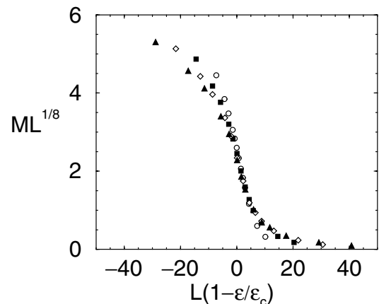
FIG. 3. Finite-size scaling function of the order parameter M with the 2D-Ising critical exponents.
