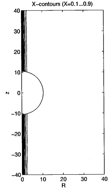
FIG. 6. Penetration of a non-extremal horizon by the Higgs field, for the values E=10 , Q=9.99 , N=1 , and \beta=1 .
