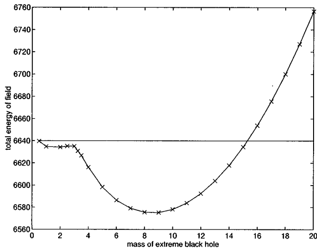
FIG. 4. Plot of total vortex field energy as a function of black hole mass.
