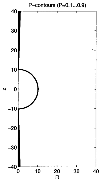
FIG. 2. Expulsion of the P field from the extreme horizon, for the values E=Q=10 , N=1 , and \beta=0.0001 .
