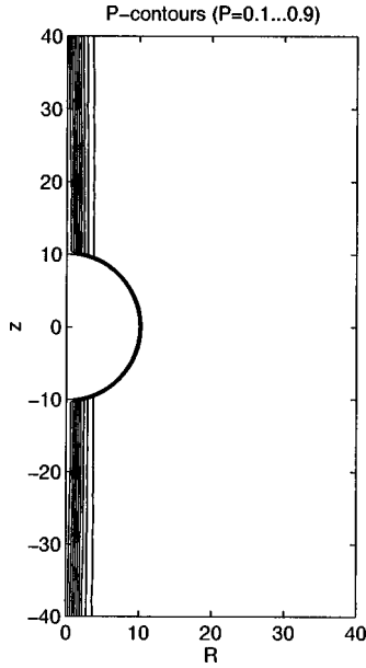
FIG. 1. Expulsion of the P field from the extreme horizon, for the values E=Q=10 , N=1 , and \beta=1 .
