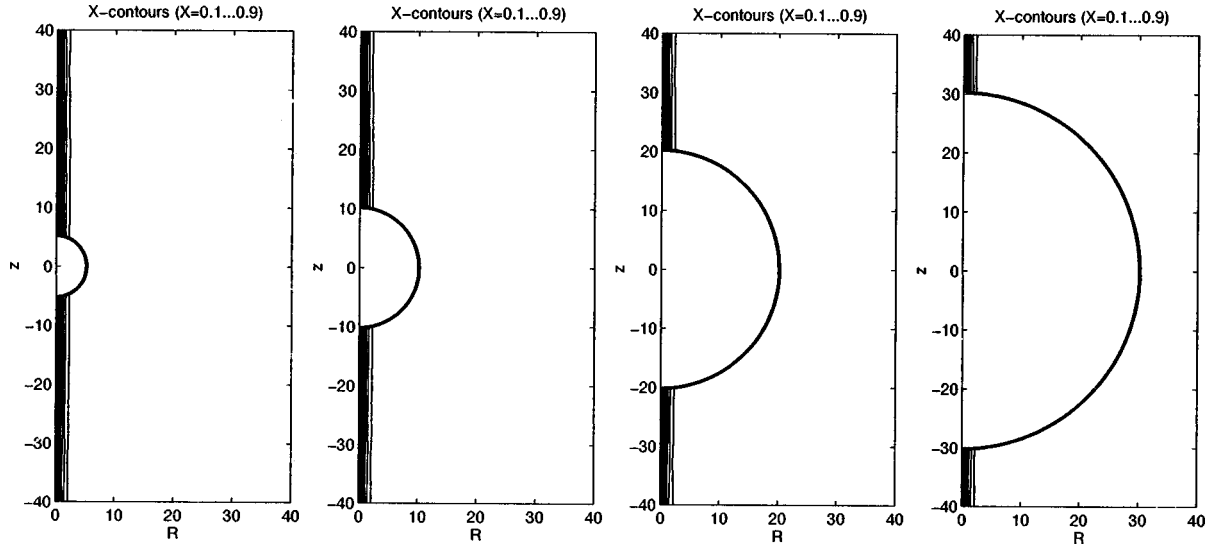
FIG. 3. Expulsion of the Higgs field from the extreme horizon, for the values (from left to right) E=Q=5,10,20,30 , N=1 , and \beta=0.5 .
