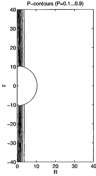
FIG. 5. Penetration of a non-extremal horizon by the P field, for the values E=10 , Q=9.99 , N=1 , and \beta=1 .
