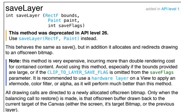
Figure 1: The documentation and deprecation message of saveLayer(RectF, Paint, int) .
